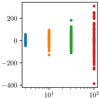
Chi Squared Distance
