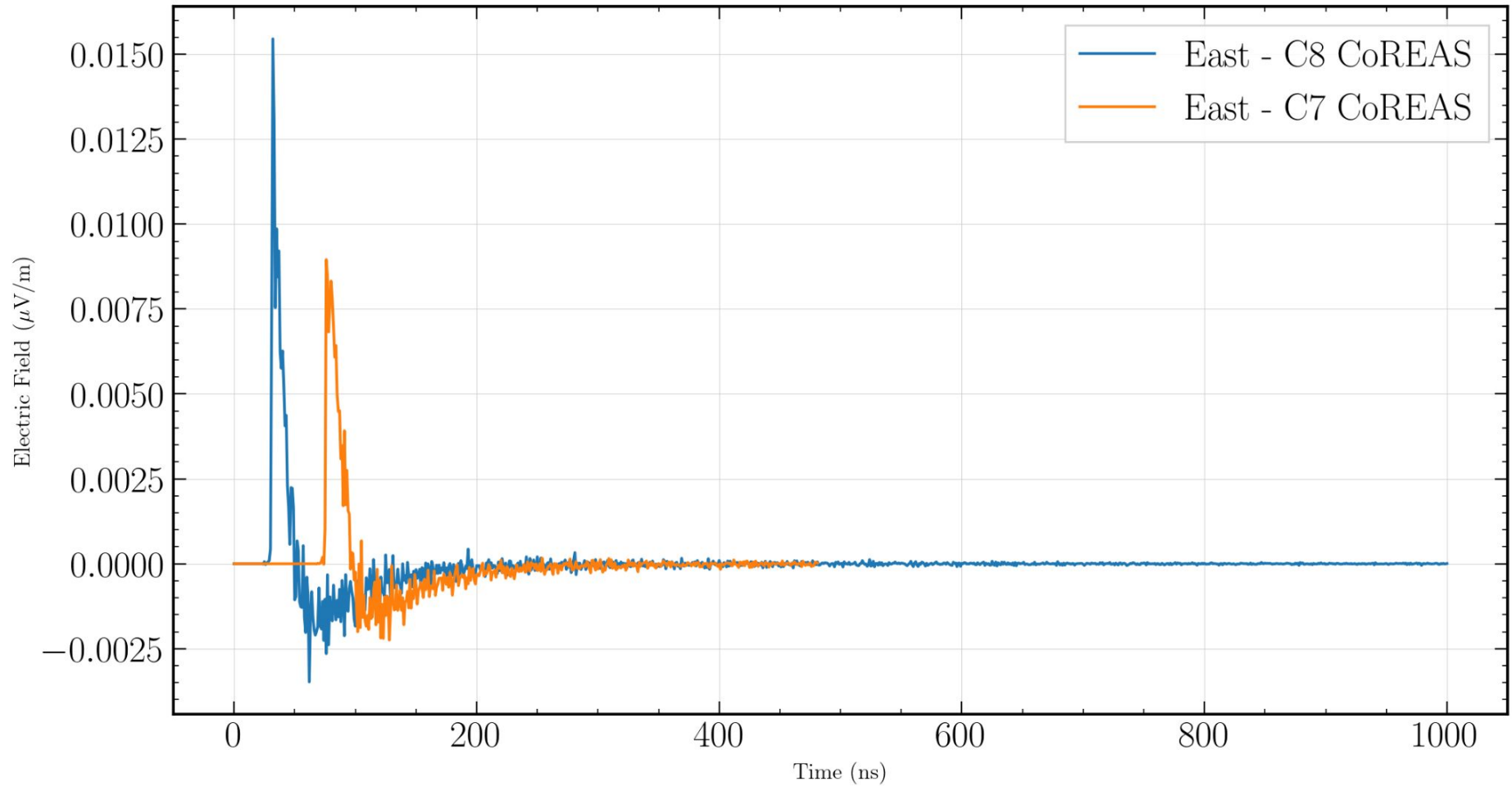
Antenna 400 m - CoREAS -
