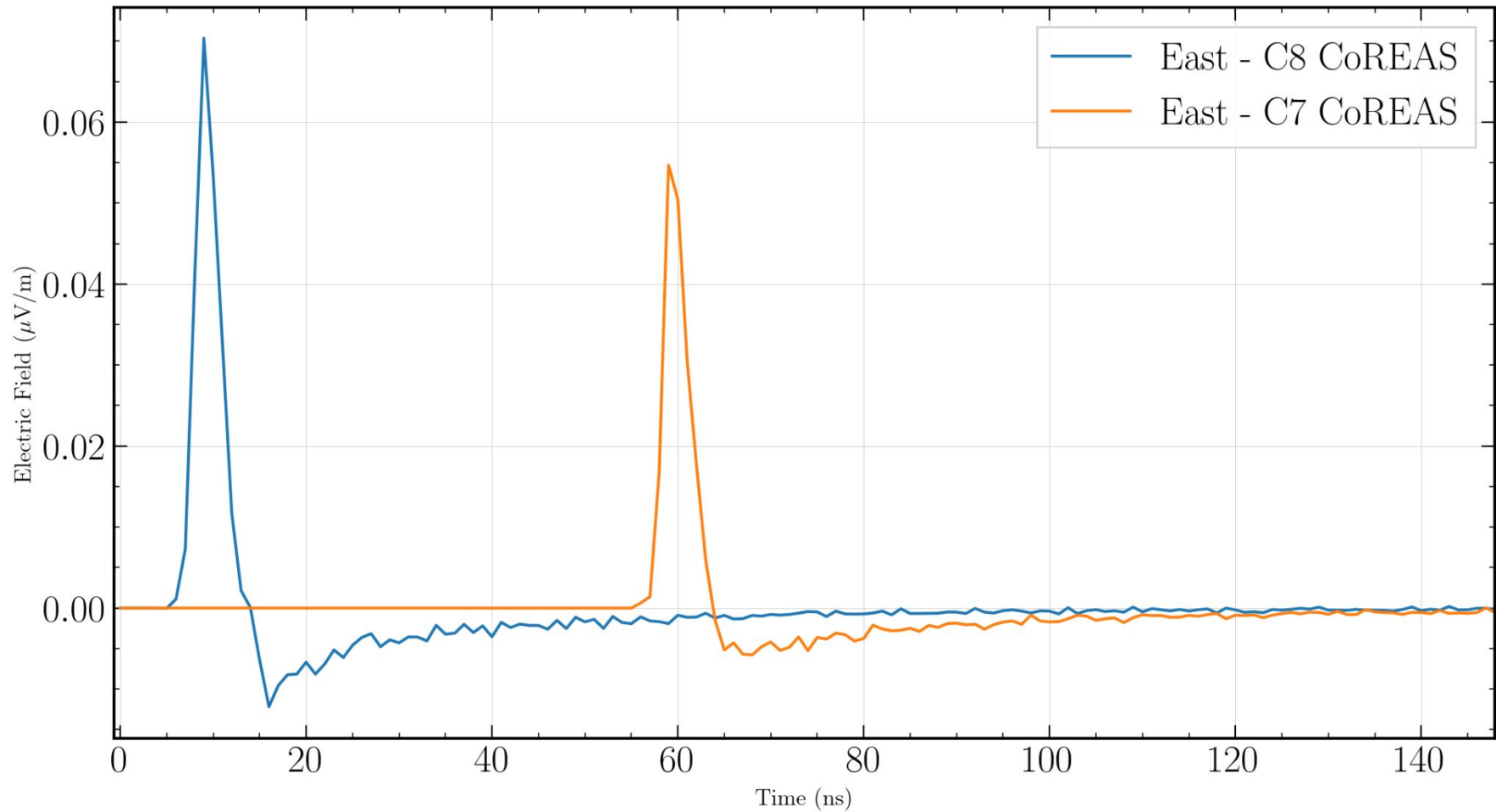
Antenna 100 m - CoREAS -
