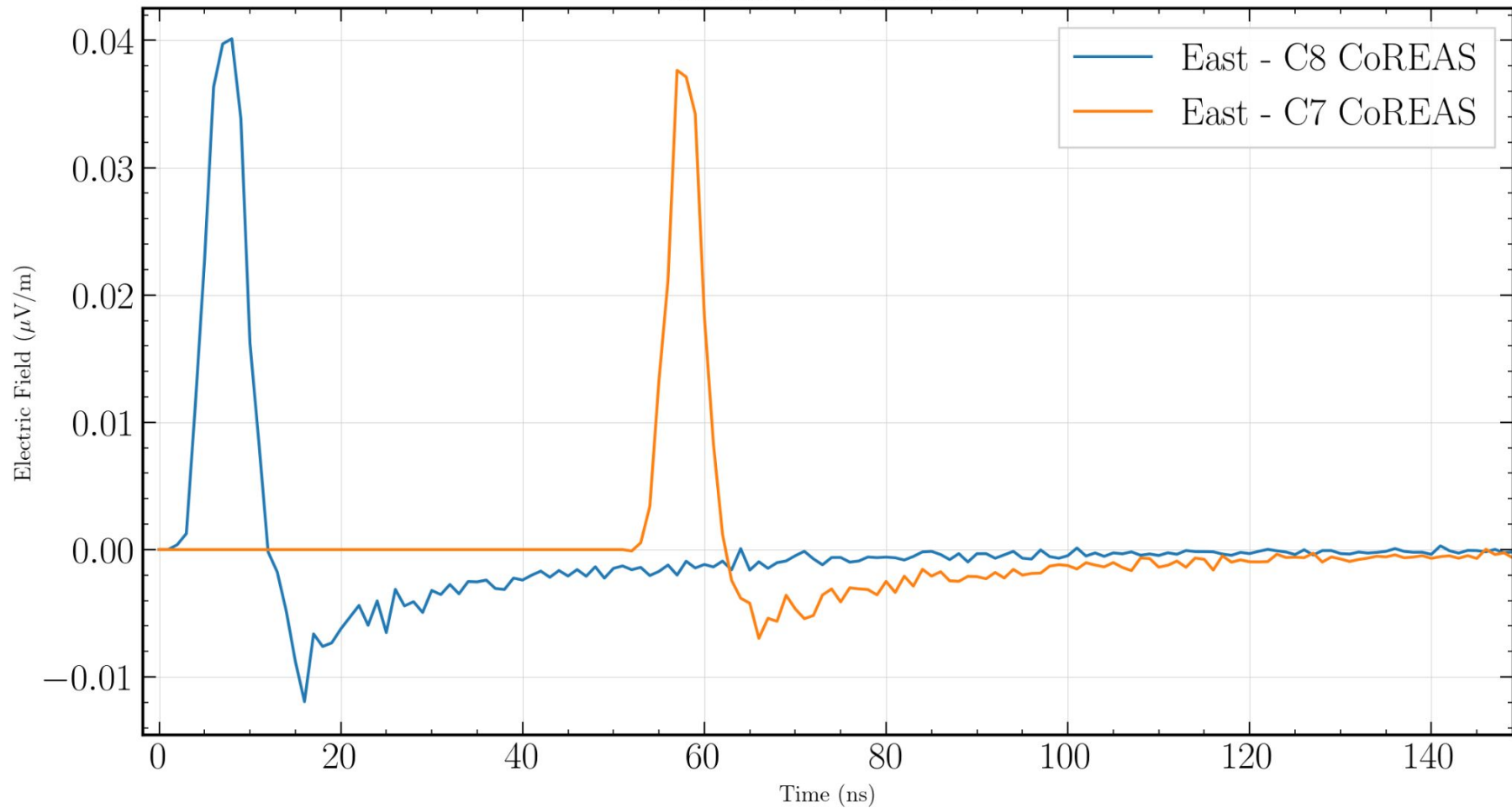
Antenna 50 m - CoREAS -
