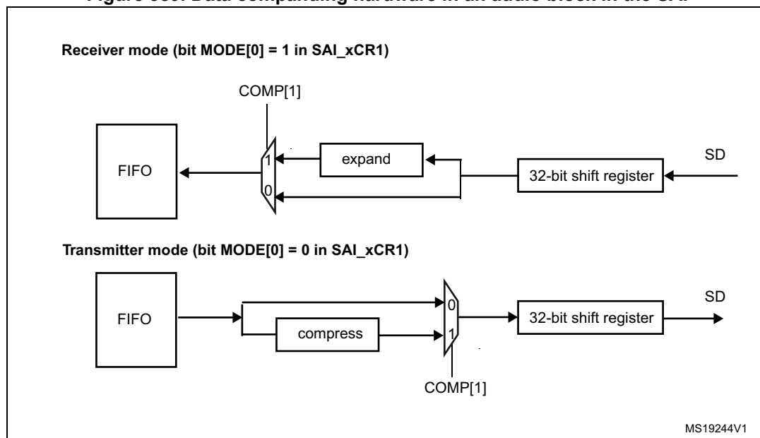
Figure 389. Data companding hardware in an audio block in the SAI
