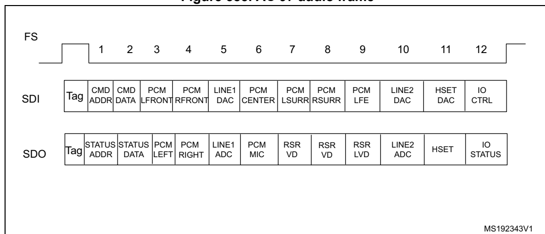
Figure 385. AC'97 audio frame
