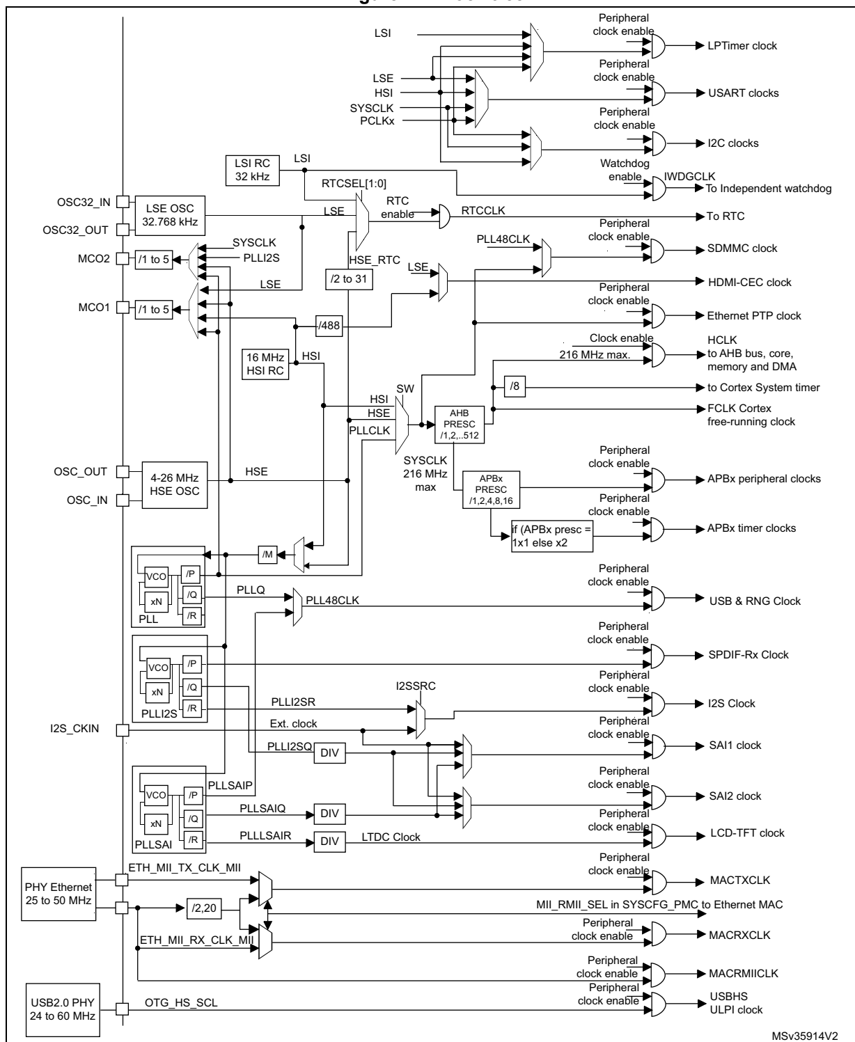
Figure 12. Clock tree
