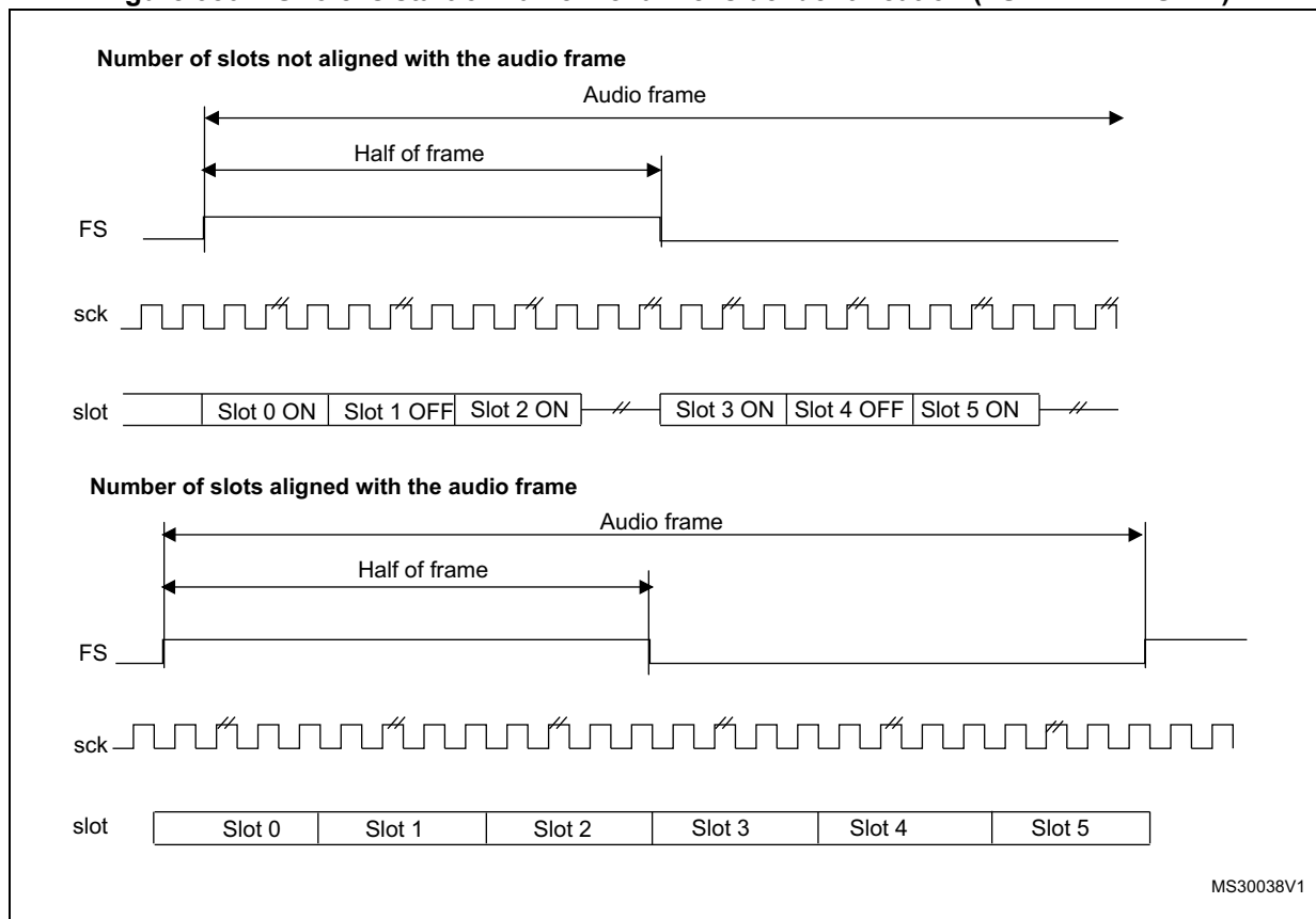
Figure 380. FS role is start of frame + channel side identification (FSDEF = TRIS = 1)
