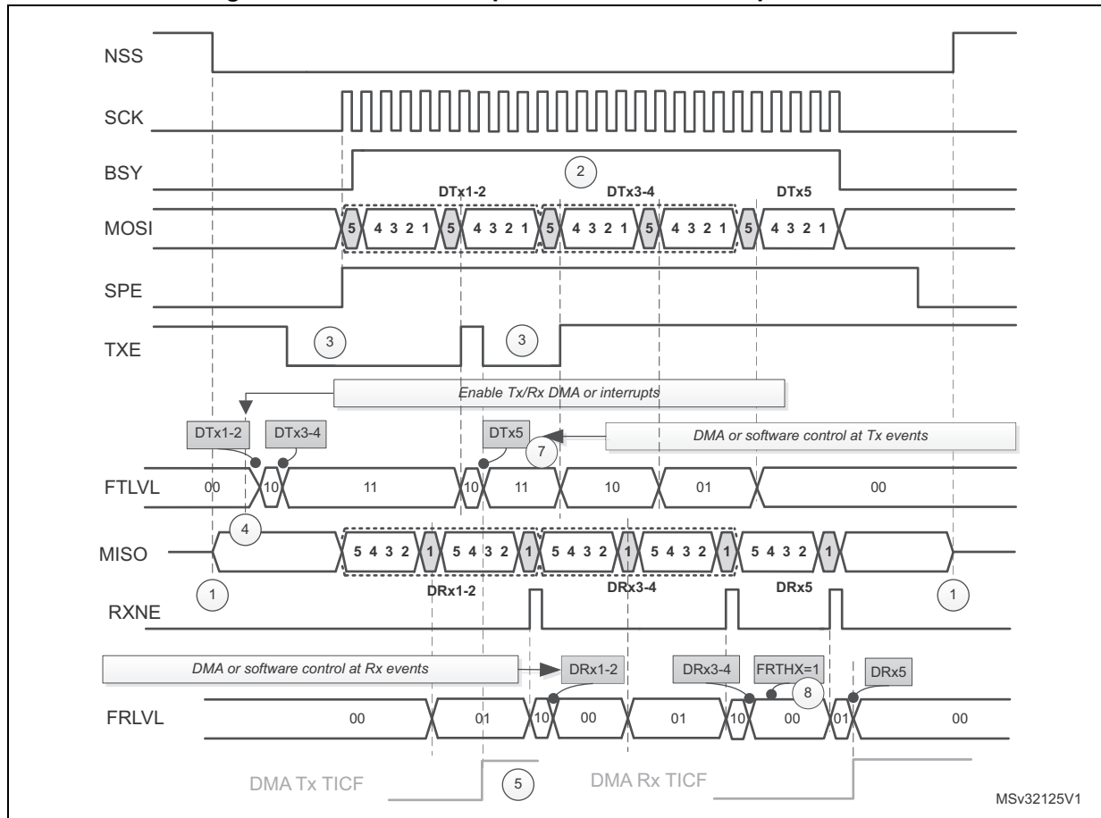
Figure 354. Master full duplex communication in packed mode
