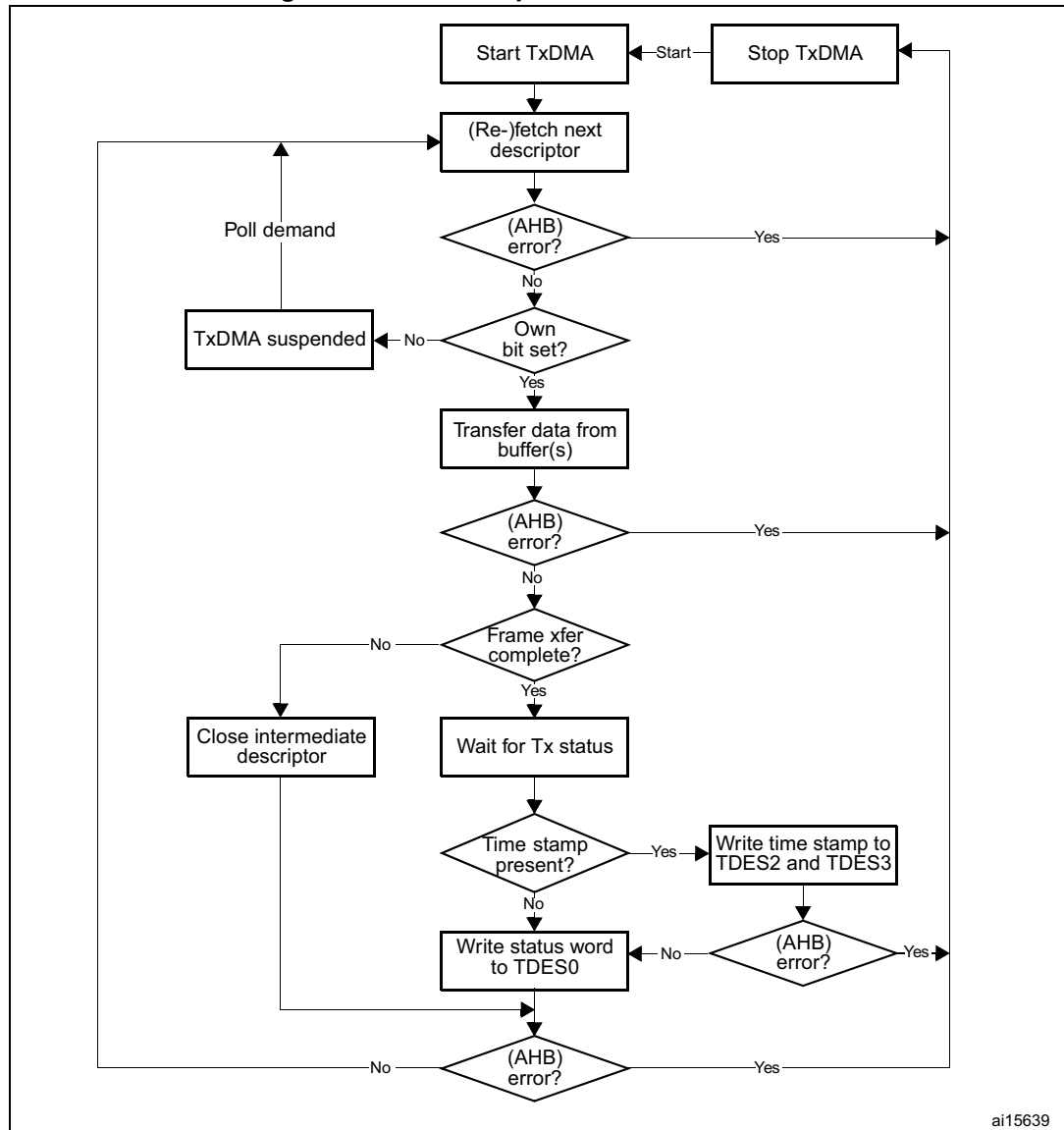
Figure 499. TxDMA operation in default mode
