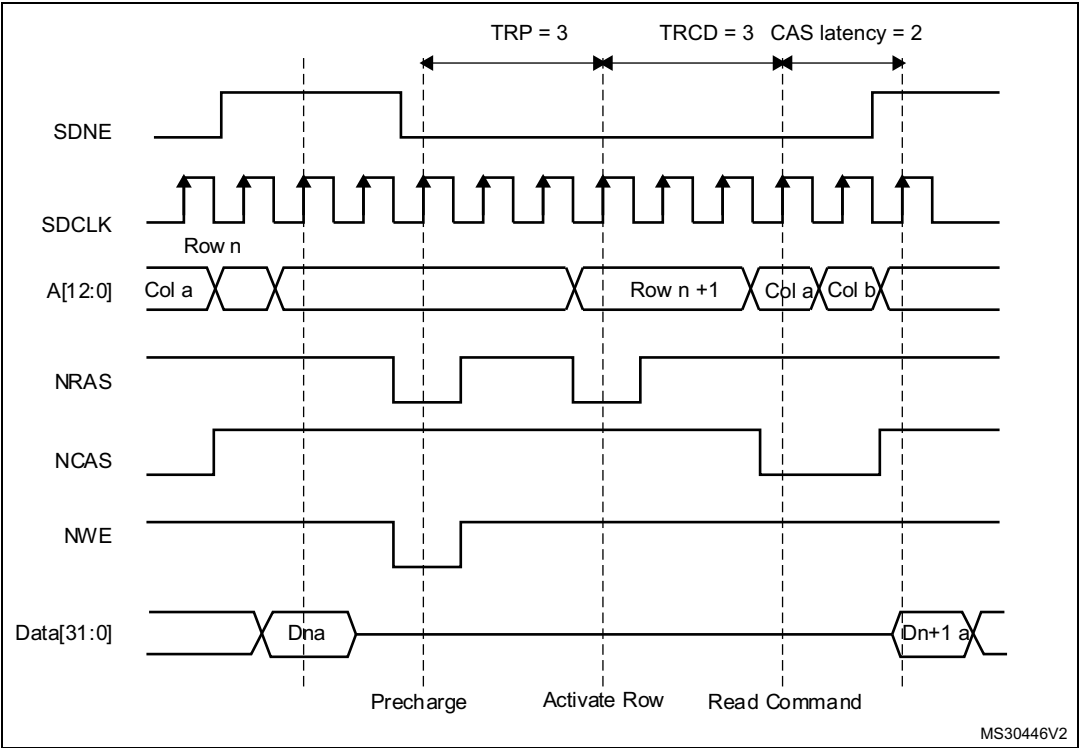
Figure 57. Read access crossing row boundary
