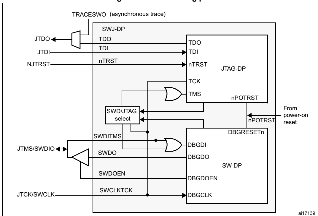
Figure 519. SWJ debug port
