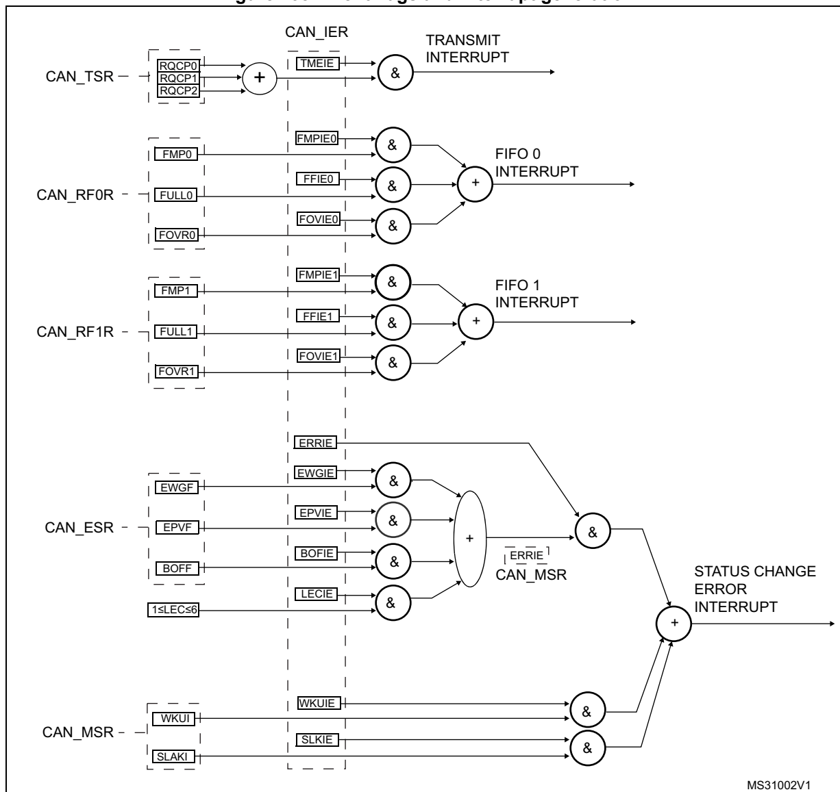
Figure 438. Event flags and interrupt generation
