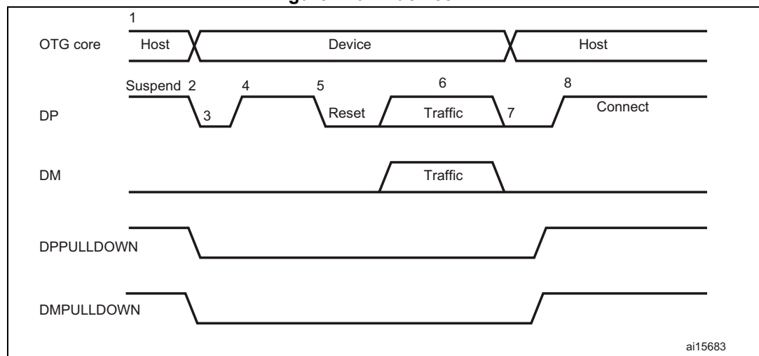
Figure 470. A-device HNP
