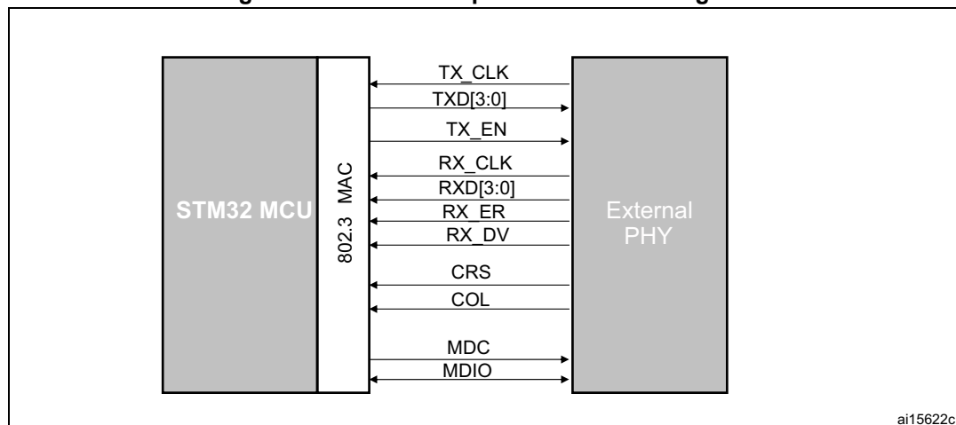
Figure 476. Media independent interface signals
