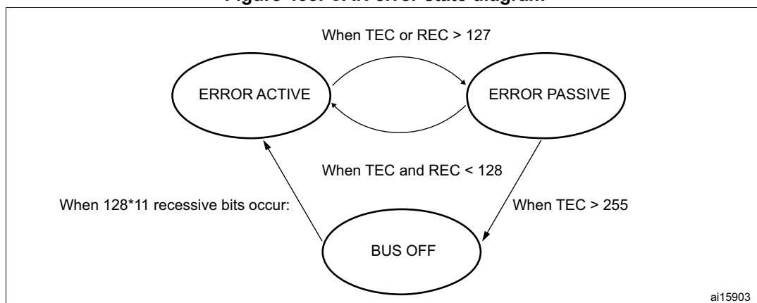
Figure 435. CAN error state diagram
