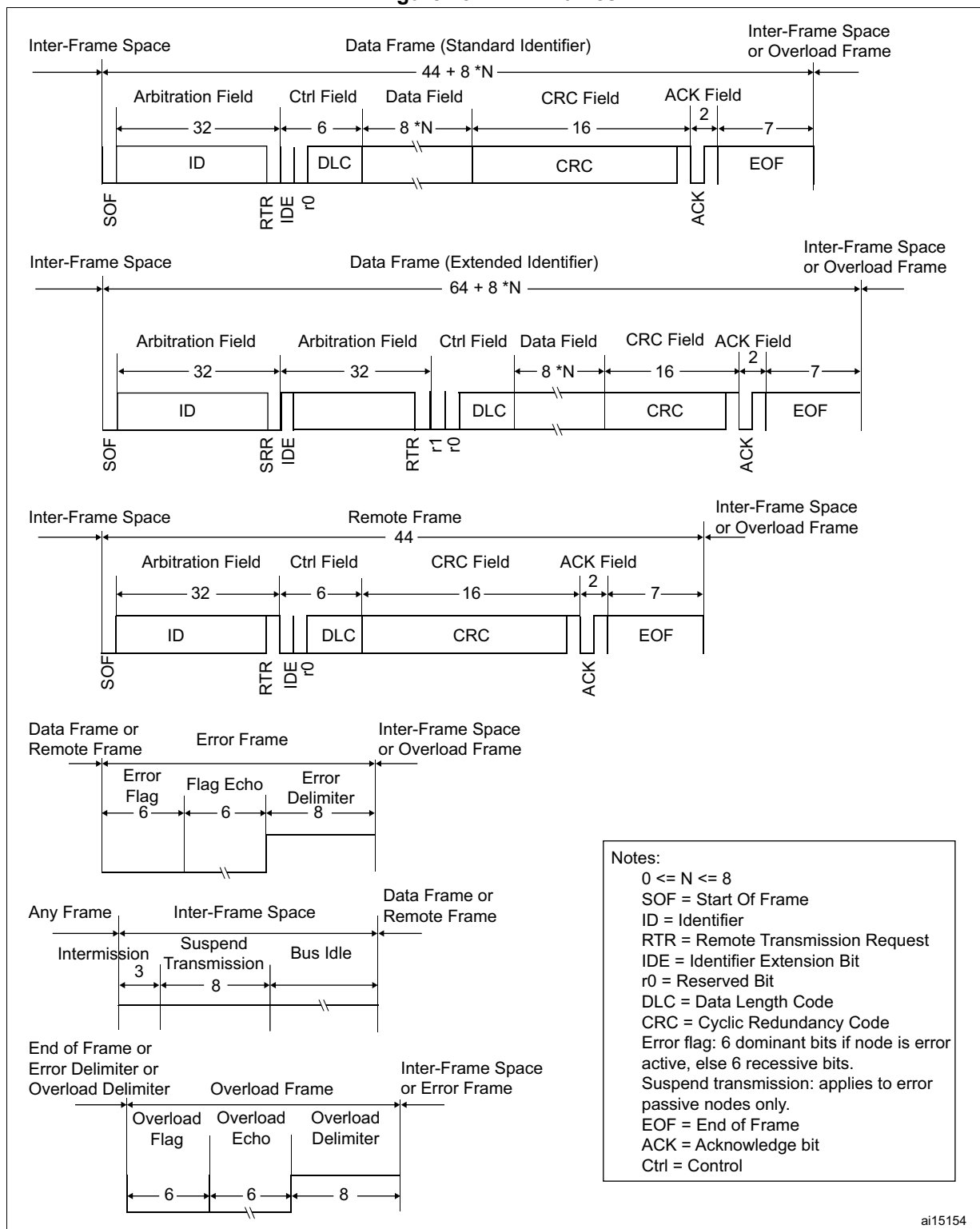
Figure 437. CAN frames
