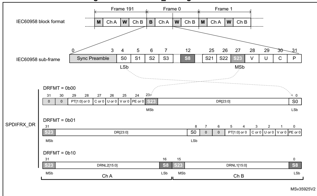
Figure 405.SPDIFRX_DR register format
