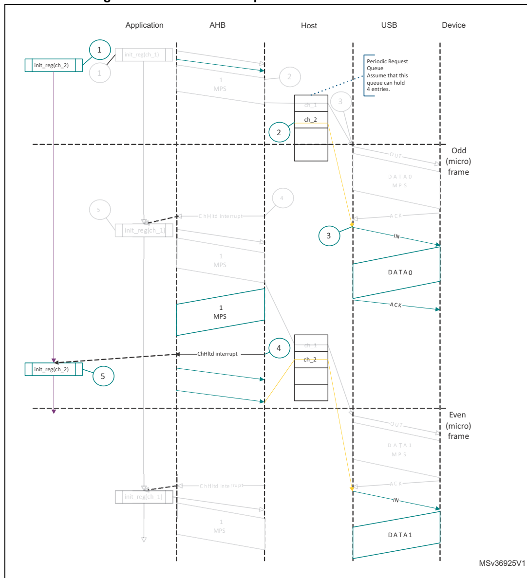
Figure 461. Normal interrupt IN transactions - DMA mode
