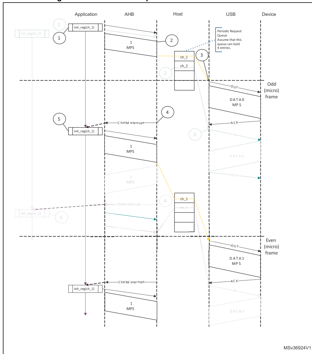
Figure 460. Normal interrupt OUT transactions - DMA mode
