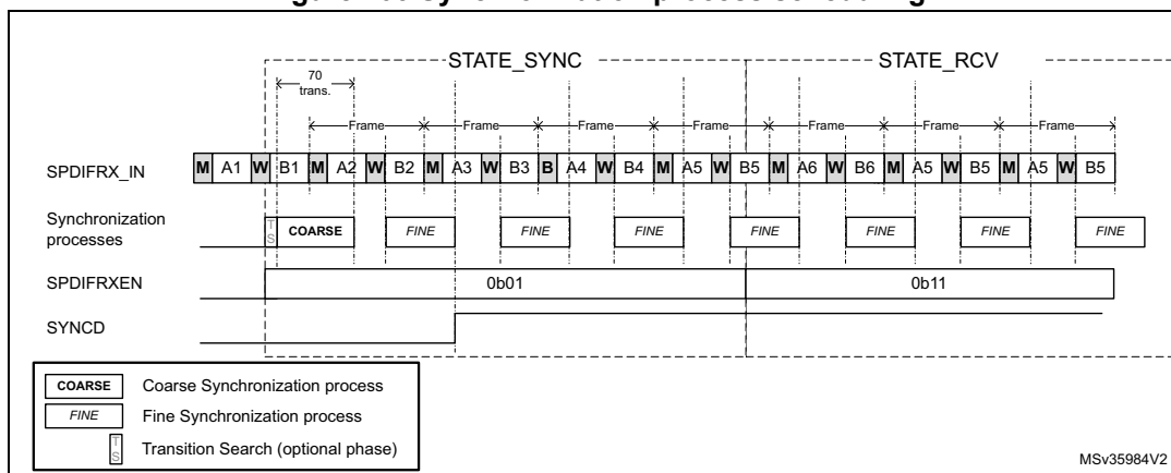
Figure 403. Synchronization process scheduling
