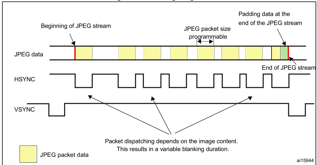
Figure 104. Timing diagram
