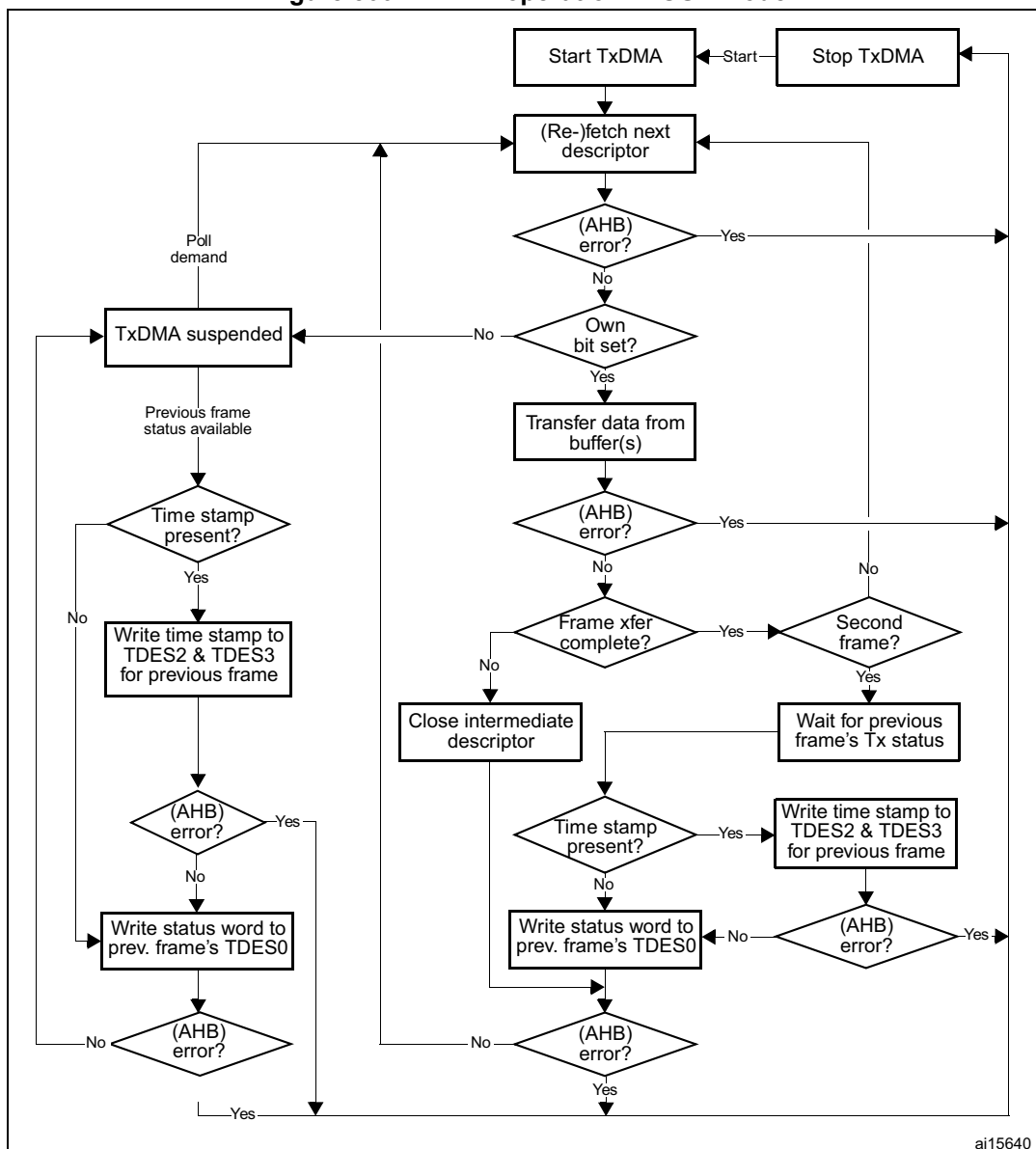
Figure 500. TxDMA operation in OSF mode
