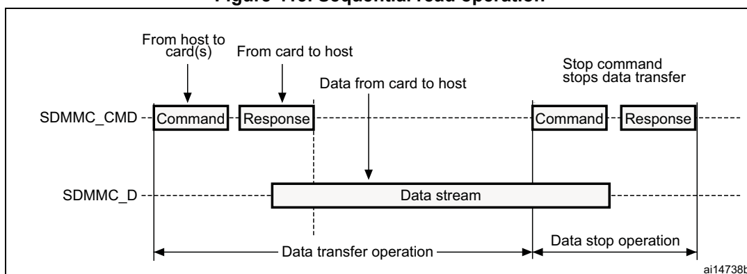
Figure 413. Sequential read operation
