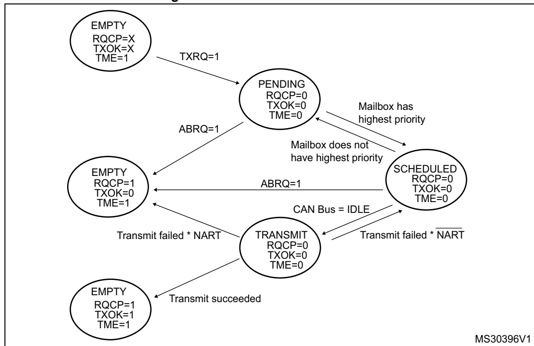
Figure 430. Transmit mailbox states
