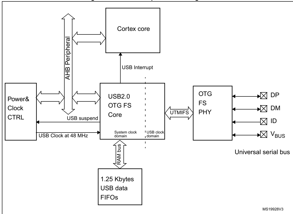
Figure 440. OTG full-speed block diagram
