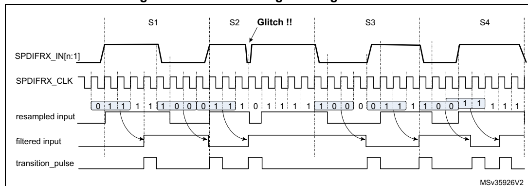
Figure 400.Noise filtering and Edge detection
