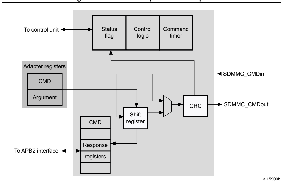
Figure 419. SDMMC adapter command path
