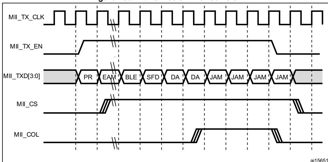
Figure 486. Transmission with collision
