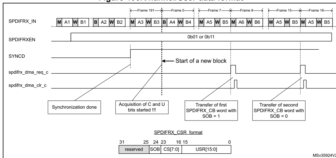
Figure 406. Channel/User data format
