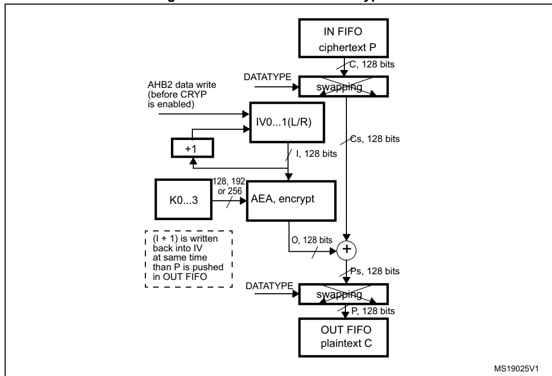
Figure 126. AES-CTR mode decryption
