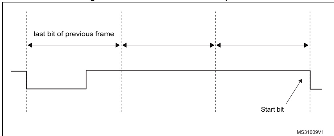
Figure 514. SFT of three nominal bit periods
