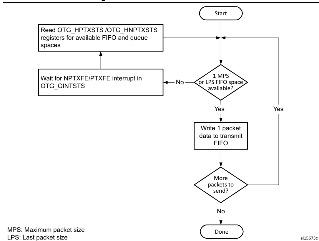
Figure 450. Transmit FIFO write task
