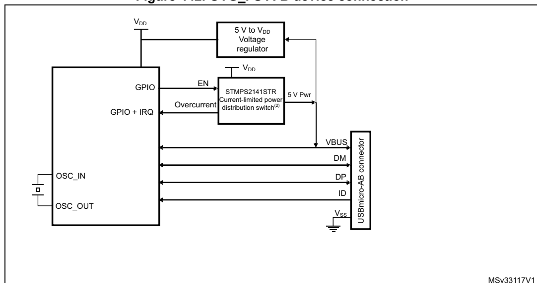
Figure 442. OTG_FS A-B device connection
