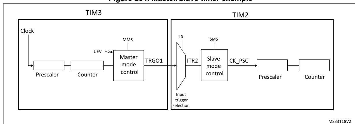
Figure 234. Master/Slave timer example
