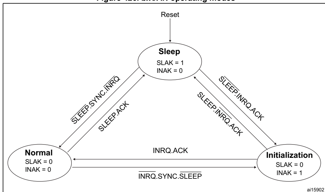
Figure 426. bxCAN operating modes
