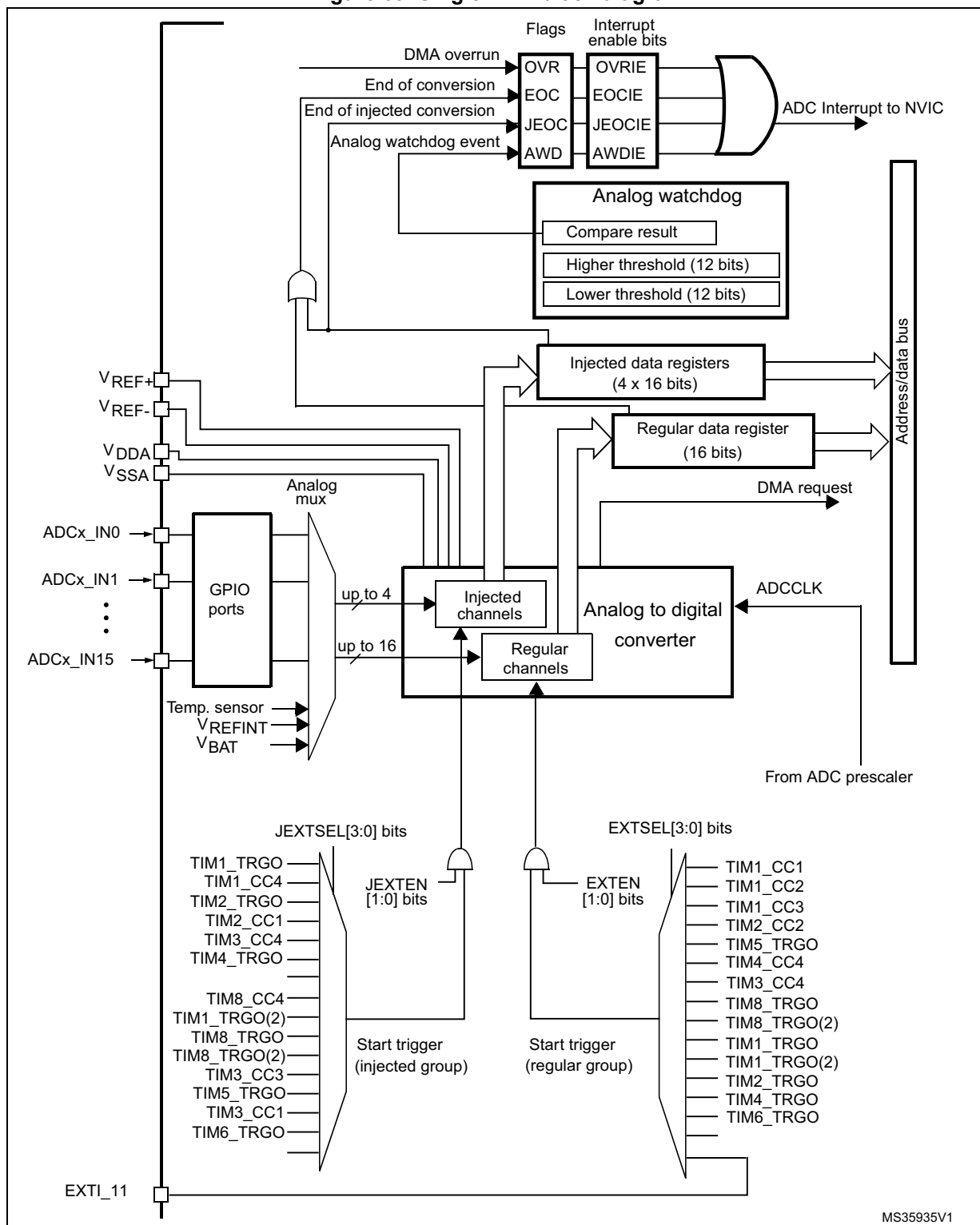
Figure 69. Single ADC block diagram
