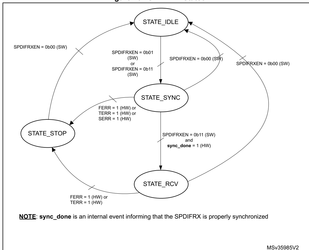
Figure 404.SPDIFRX States
