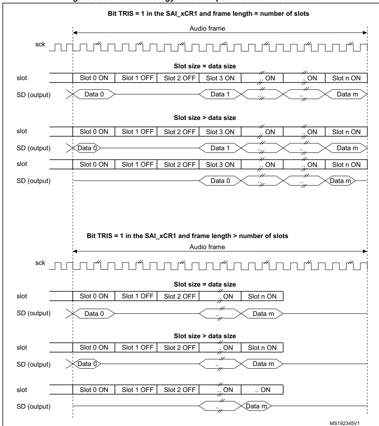
Figure 390. Tristate strategy on SD output line on an inactive slot
