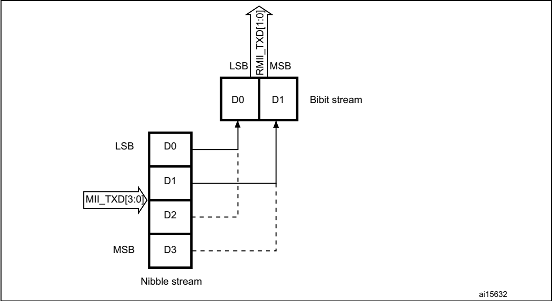
Figure 484. Transmission bit order
