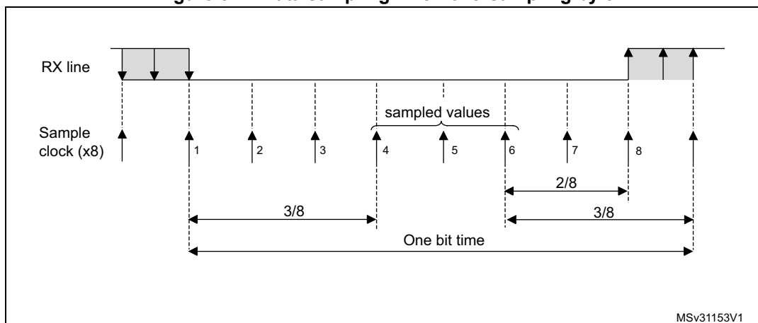
Figure 322. Data sampling when oversampling by 8
