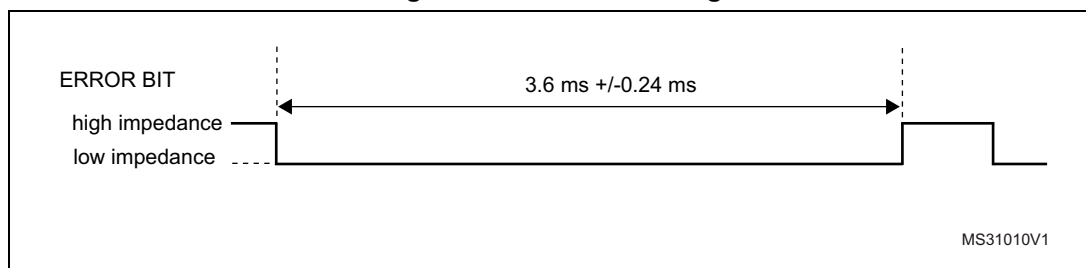
Figure 515. Error bit timing
