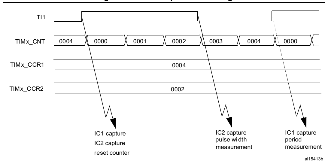
Figure 256. PWM input mode timing
