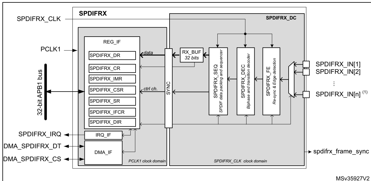
Figure 394.SPDIFRX block diagram
