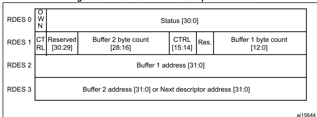
Figure 504. Normal Rx DMA descriptor structure
