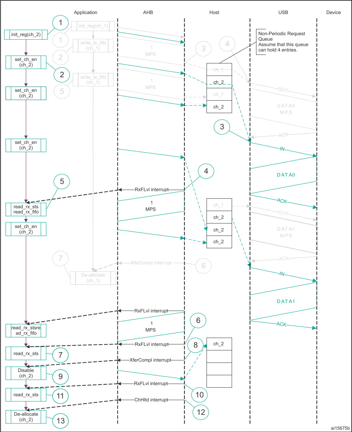
Figure 453. Bulk/control IN transactions
