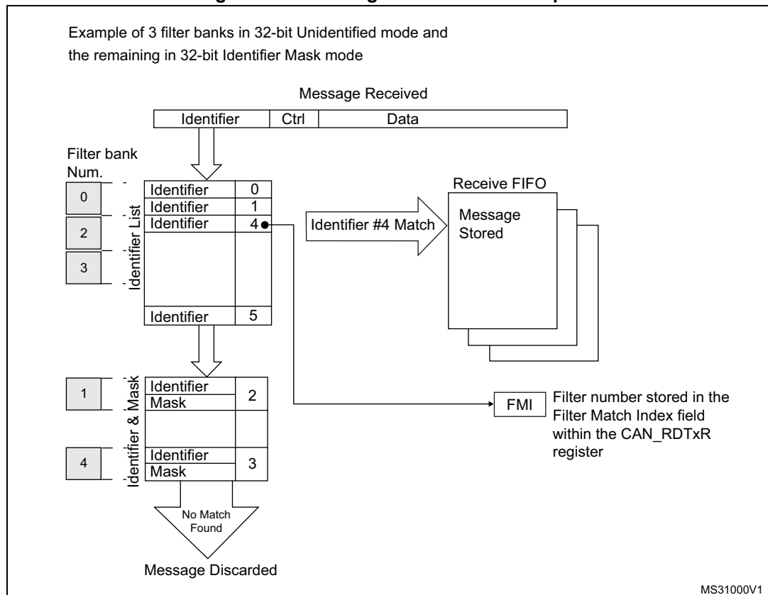
Figure 434. Filtering mechanism - example
