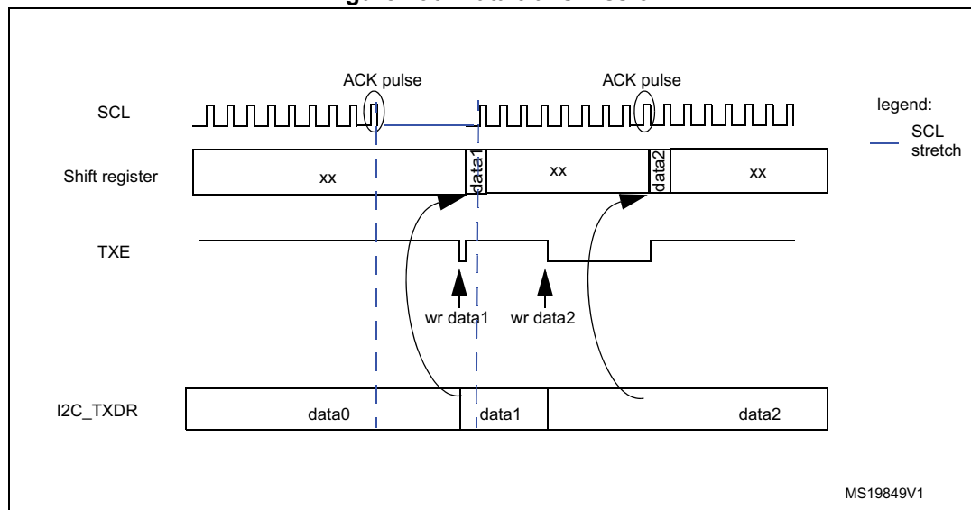
Figure 290. Data transmission
