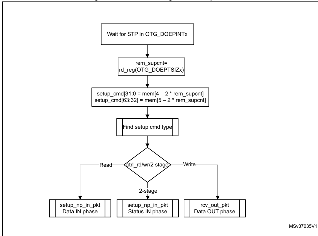
Figure 465. Processing a SETUP packet
