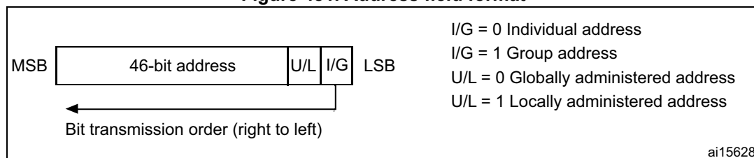
Figure 481. Address field format
