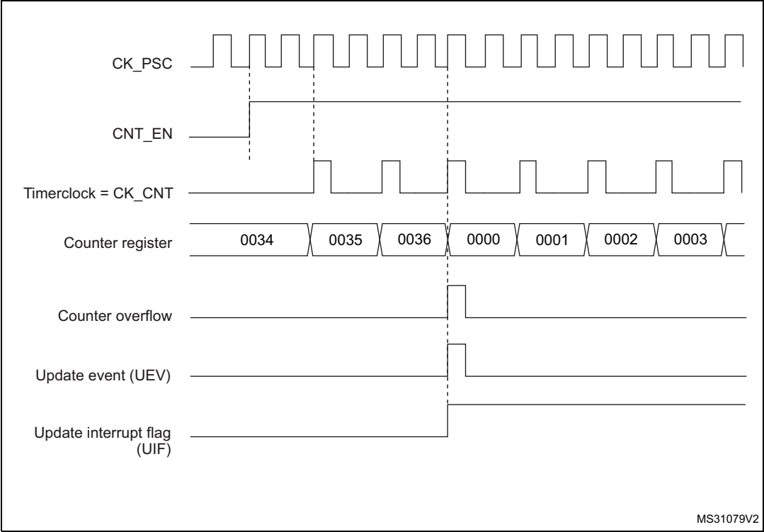
Figure 245. Counter timing diagram, internal clock divided by 2
