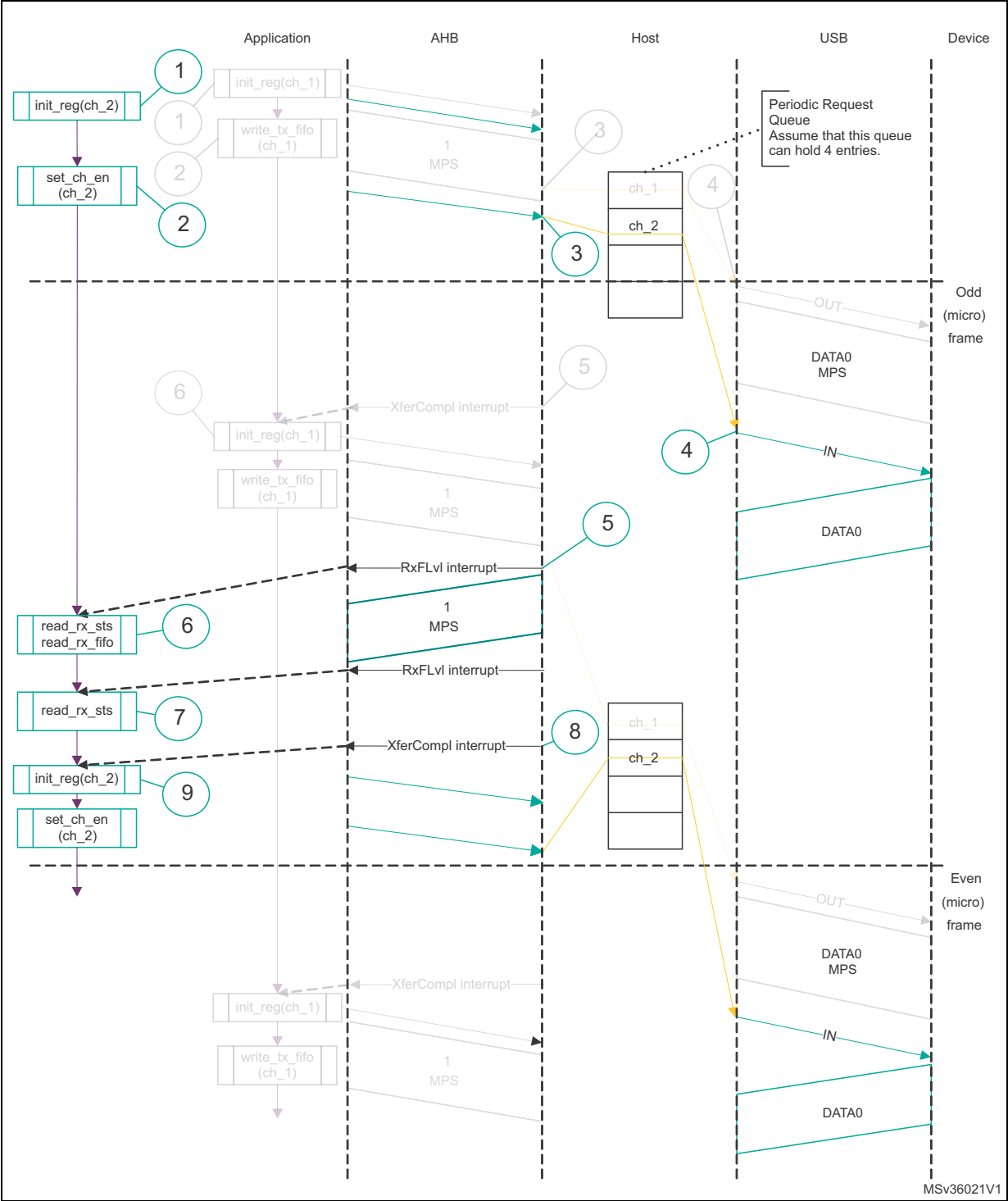
Figure 457. Isochronous IN transactions
