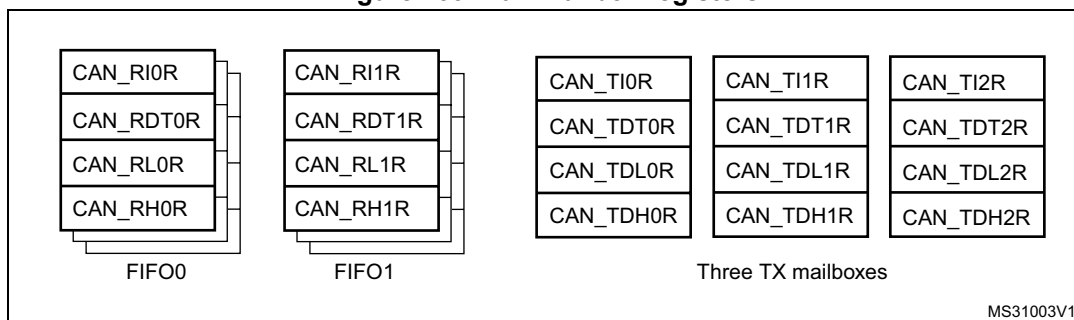
Figure 439. Can mailbox registers
