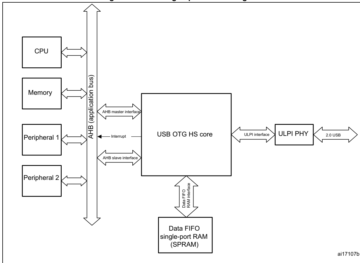
Figure 441. OTG high-speed block diagram
