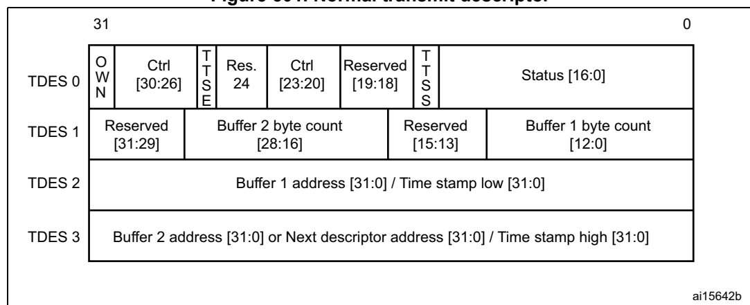
Figure 501. Normal transmit descriptor
