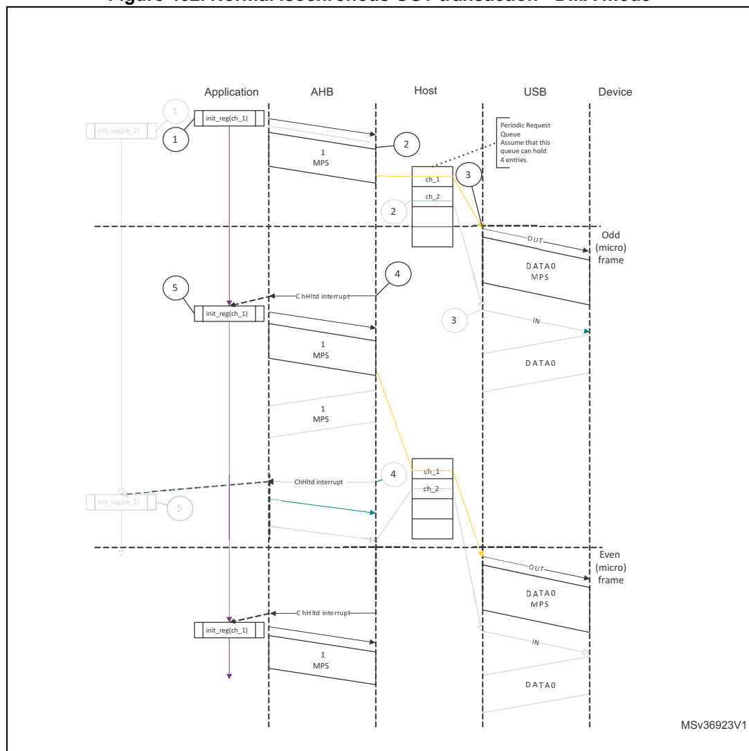
Figure 462. Normal isochronous OUT transaction - DMA mode
