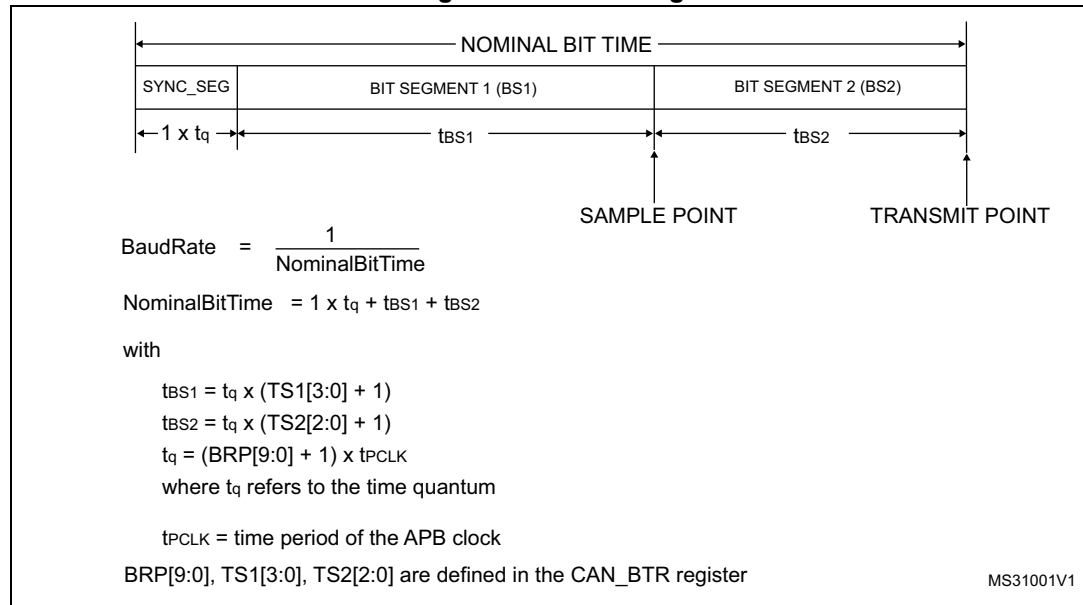
Figure 436. Bit timing
