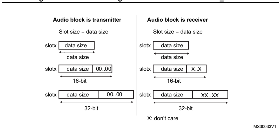
Figure 382. Slot size configuration with FBOFF = 0 in SAI_xSLOTR
