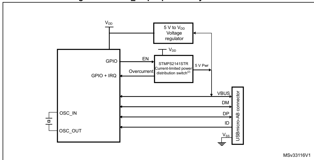
Figure 443. USB_FS peripheral-only connection
