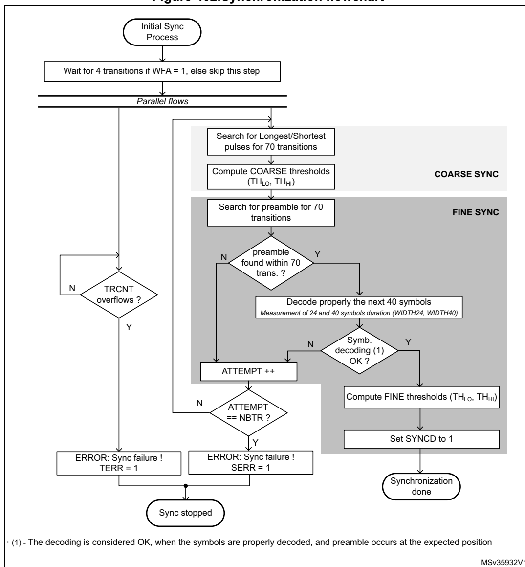
Figure 402. Synchronization flowchart
