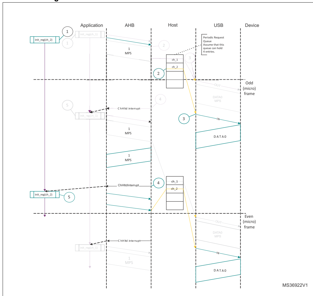
Figure 463. Normal isochronous IN transactions - DMA mode
