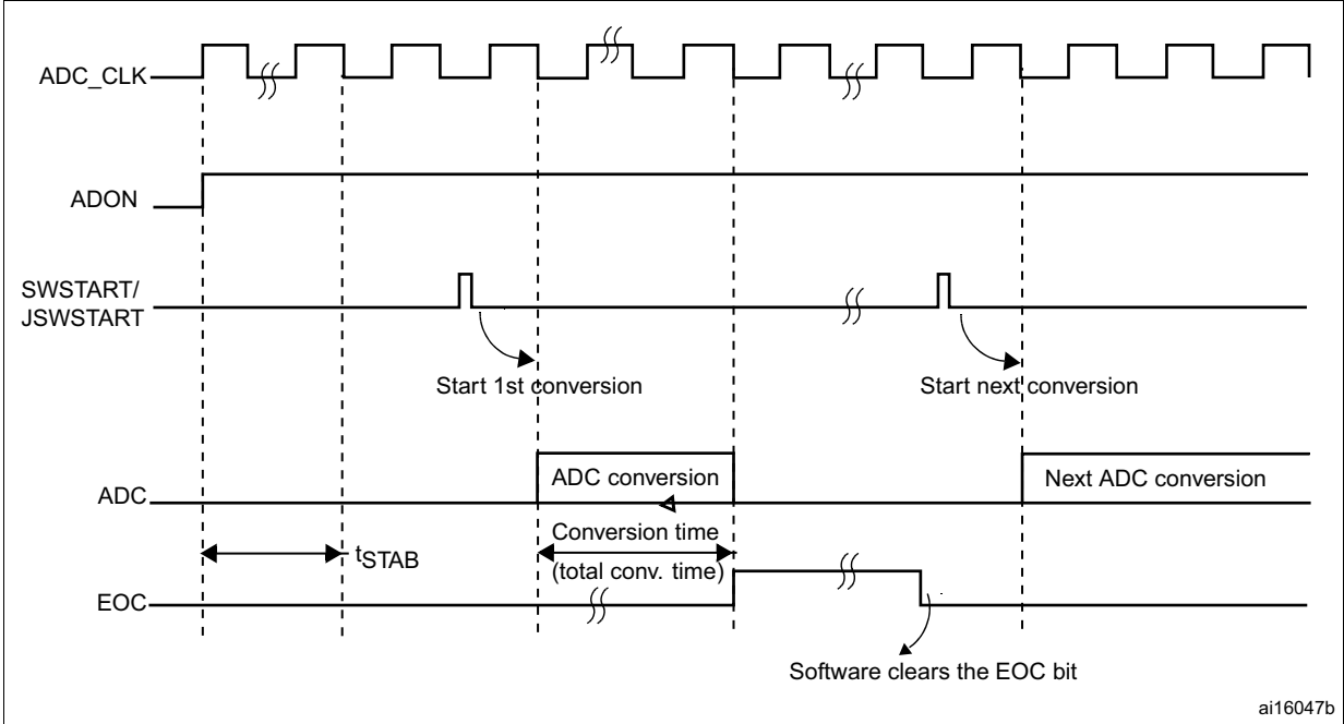
Figure 73. Timing diagram
