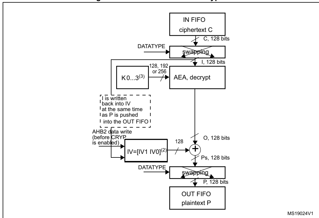
Figure 124. AES-CBC mode decryption
