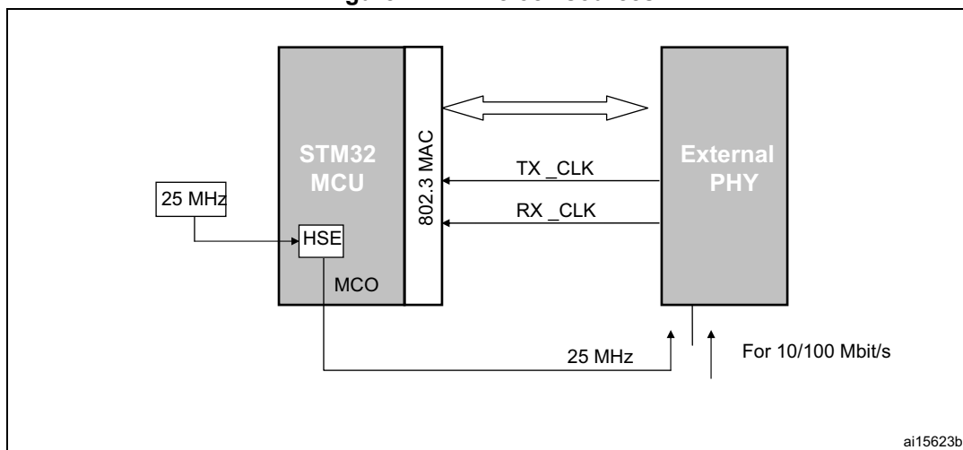
Figure 477. MII clock sources
