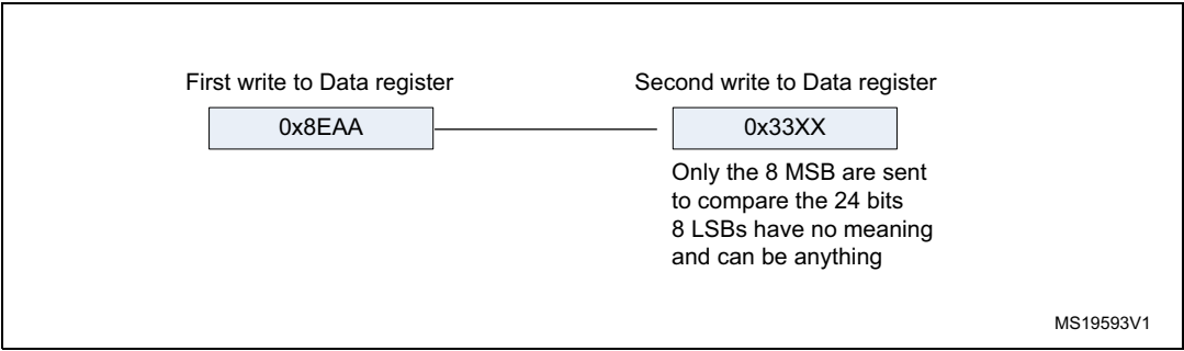
Figure 360. Transmitting 0x8EAA33
