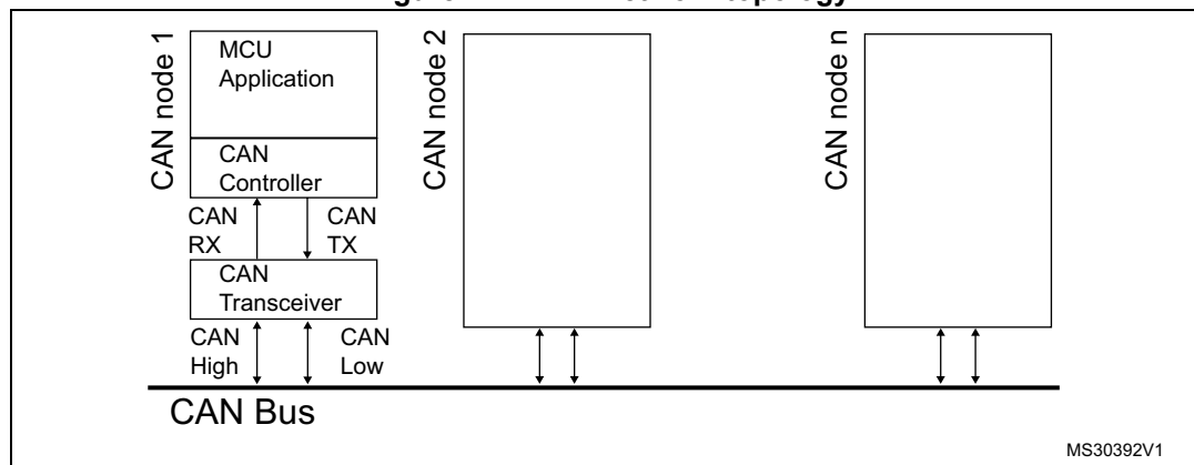
Figure 424. CAN network topology
