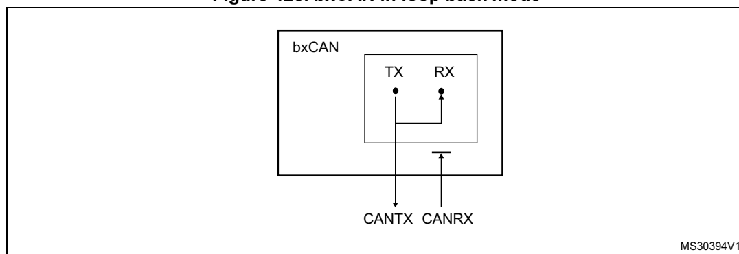
Figure 428. bxCAN in loop back mode
