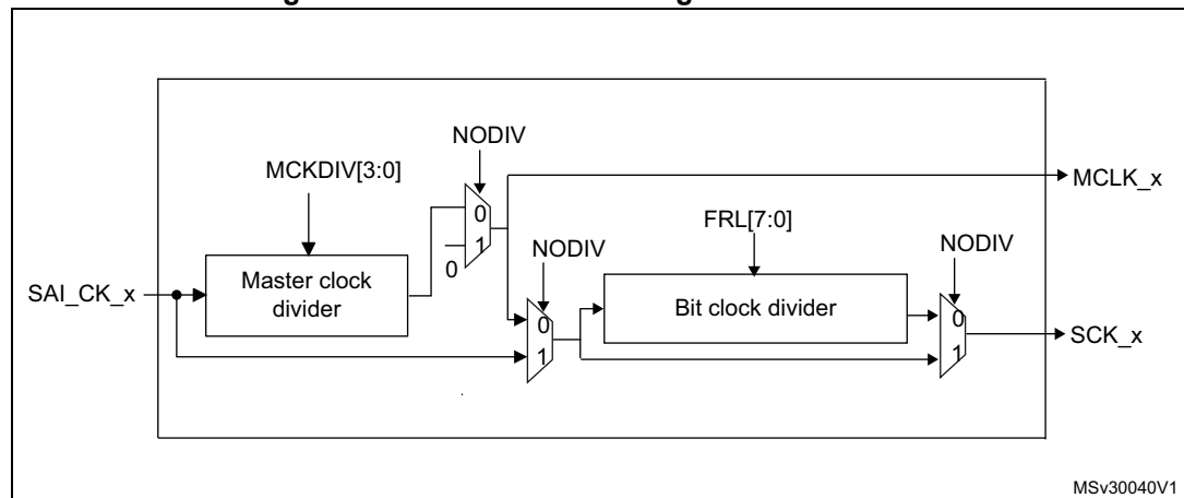
Figure 384. Audio block clock generator overview
