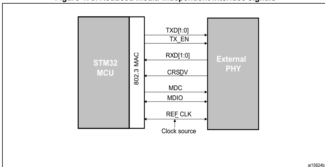
Figure 478. Reduced media-independent interface signals
