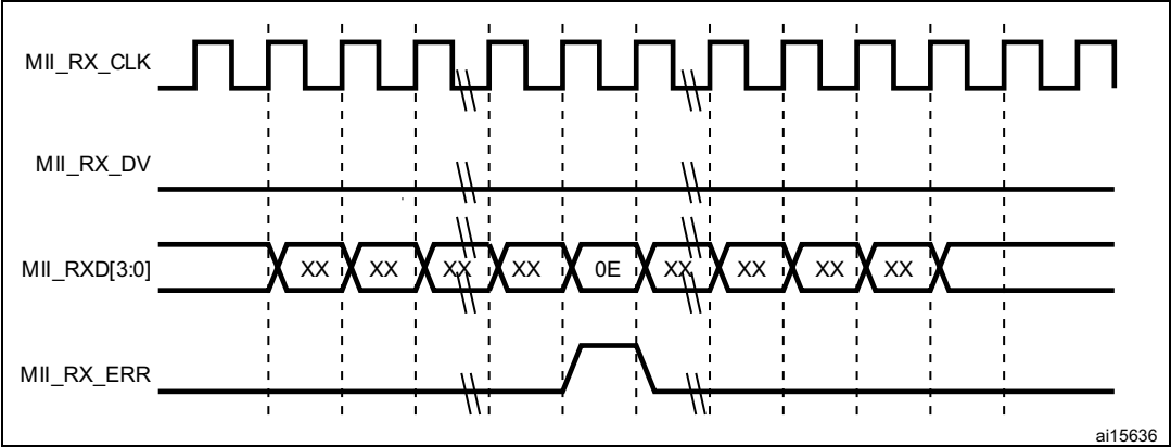
Figure 491. Reception with false carrier indication
