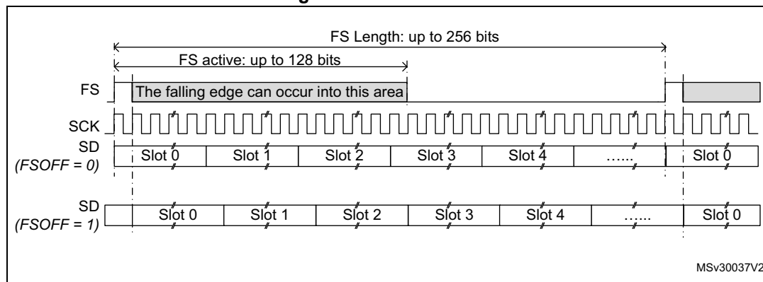
Figure 379. Audio frame
