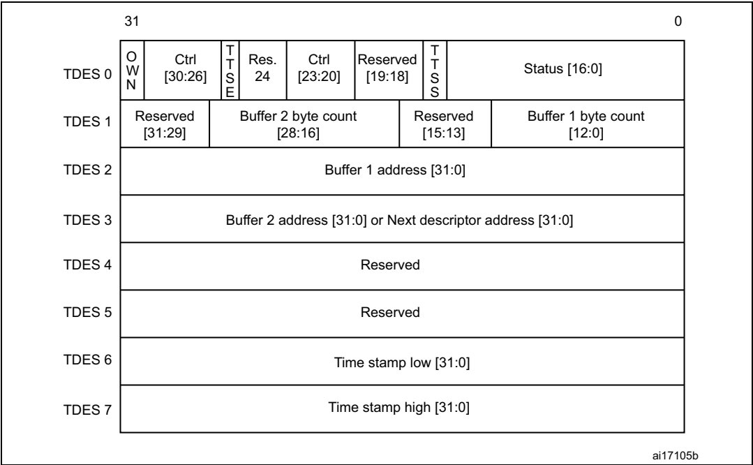
Figure 502. Enhanced transmit descriptor
