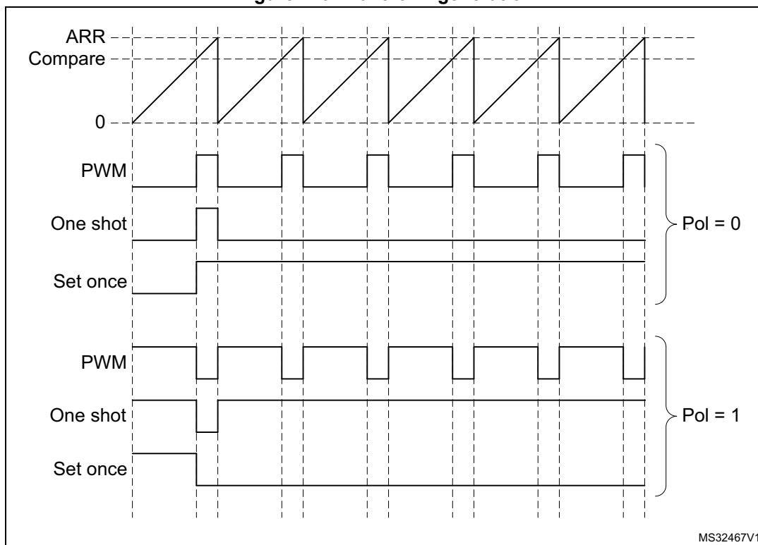
Figure 279. Waveform generation
