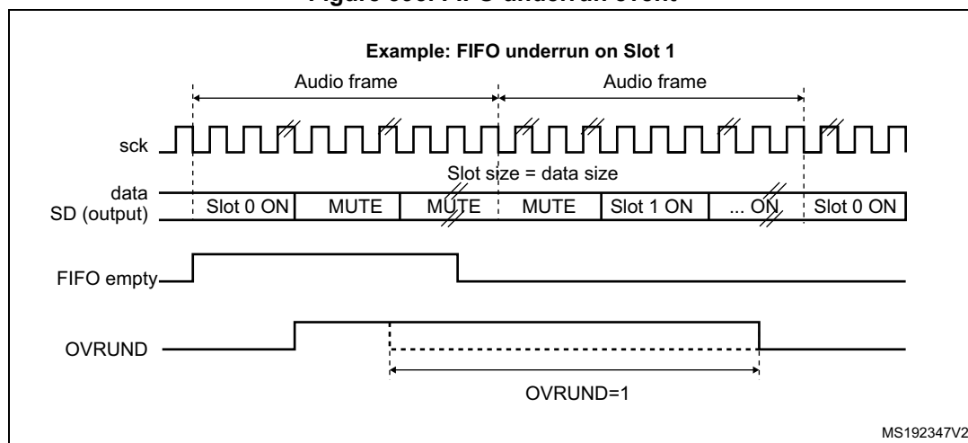
Figure 393. FIFO underrun event
