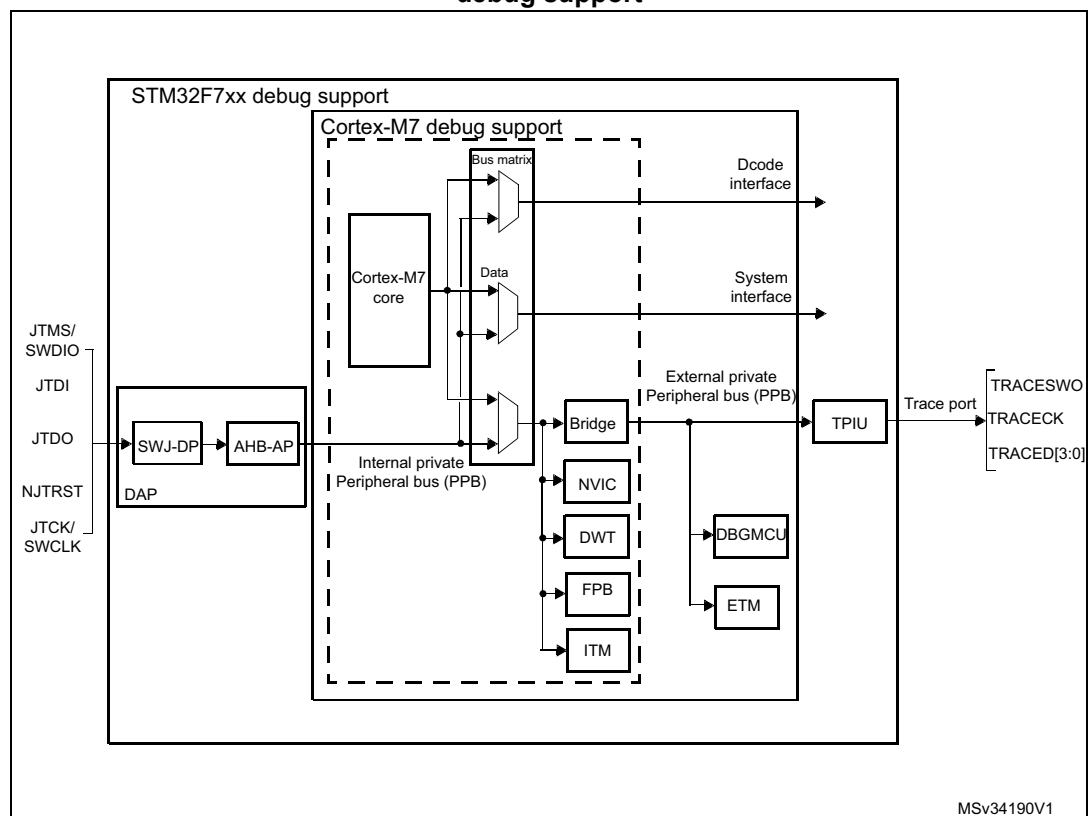
Figure 518. Block diagram of STM32 MCU and Cortex®-M7 with FPU -level debug support
