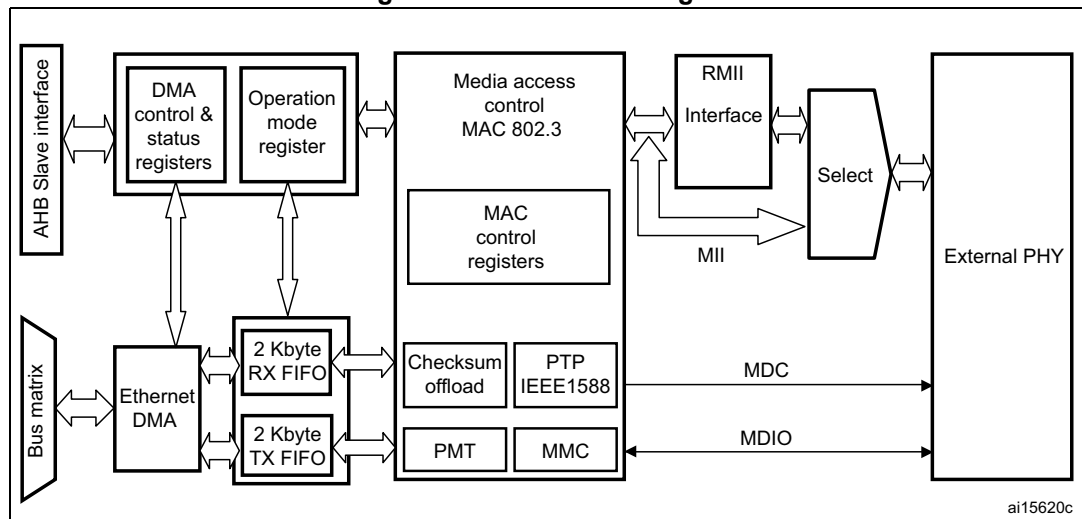
Figure 472. ETH block diagram
