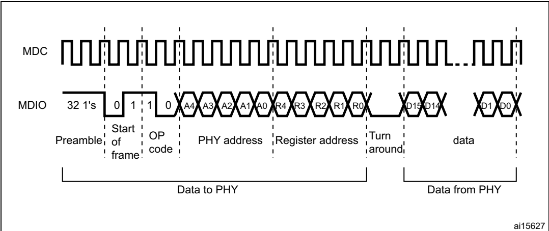
Figure 475. MDIO timing and frame structure - Read cycle
