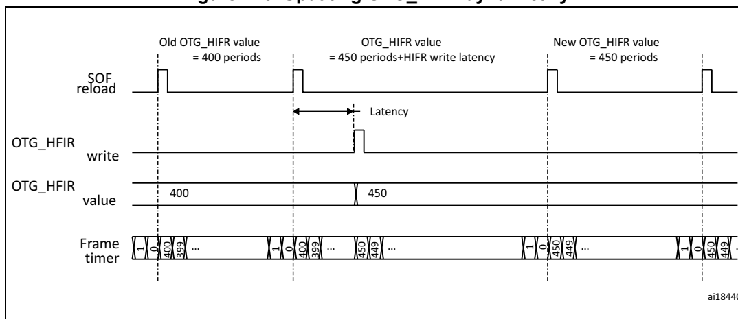
Figure 446. Updating OTG_HFIR dynamically
