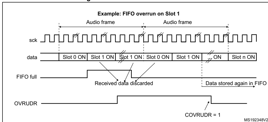
Figure 392. Overrun detection error
