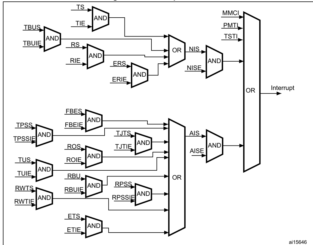
Figure 506. Interrupt scheme
