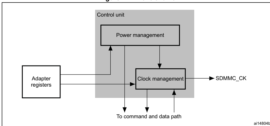
Figure 417. Control unit
