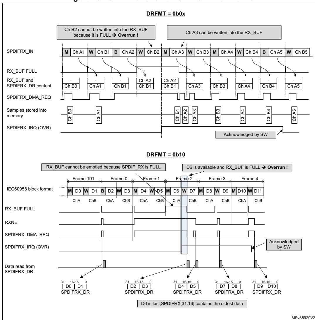
Figure 407. S/PDIF overrun error when RXSTEO = 0
