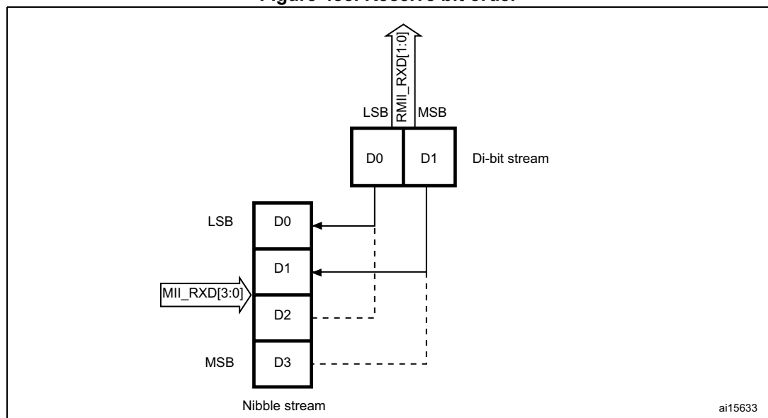
Figure 488. Receive bit order
