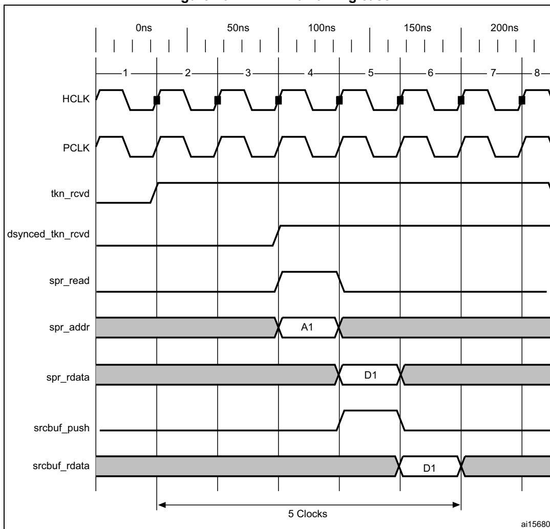
Figure 467. TRDT max timing case
