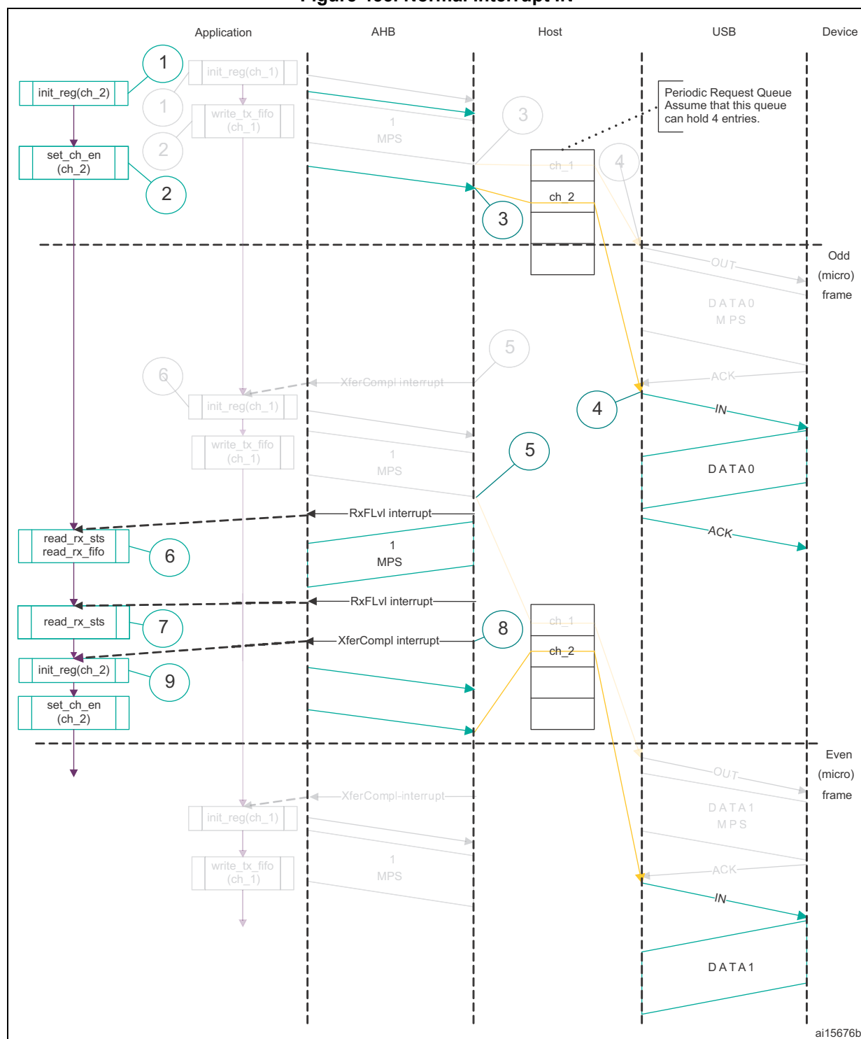
Figure 455. Normal interrupt IN
