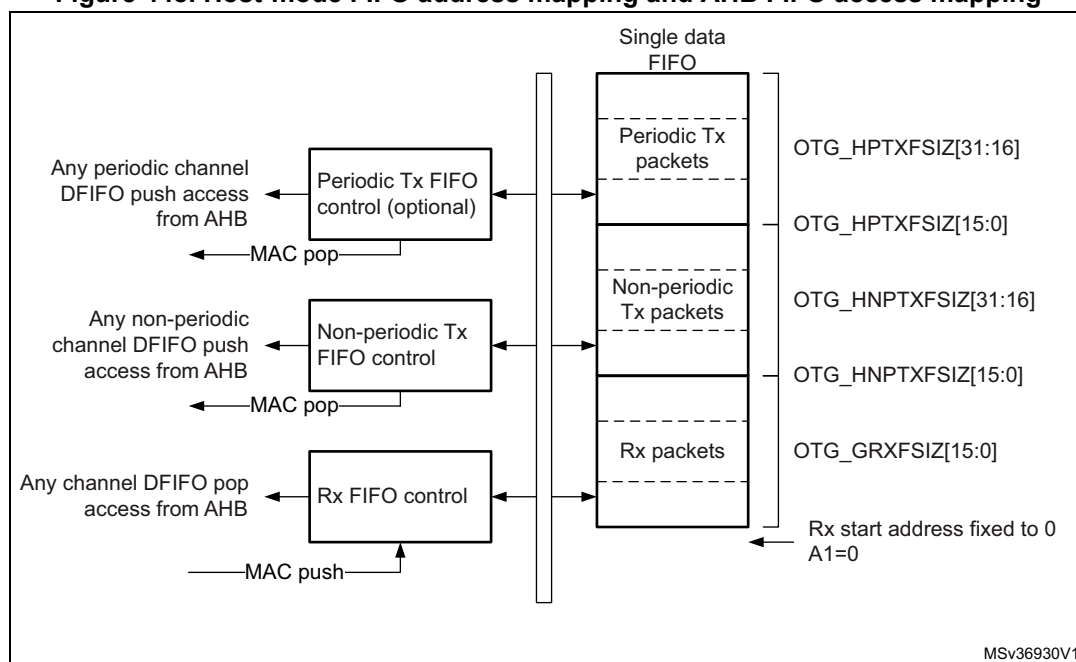
Figure 448. Host-mode FIFO address mapping and AHB FIFO access mapping
