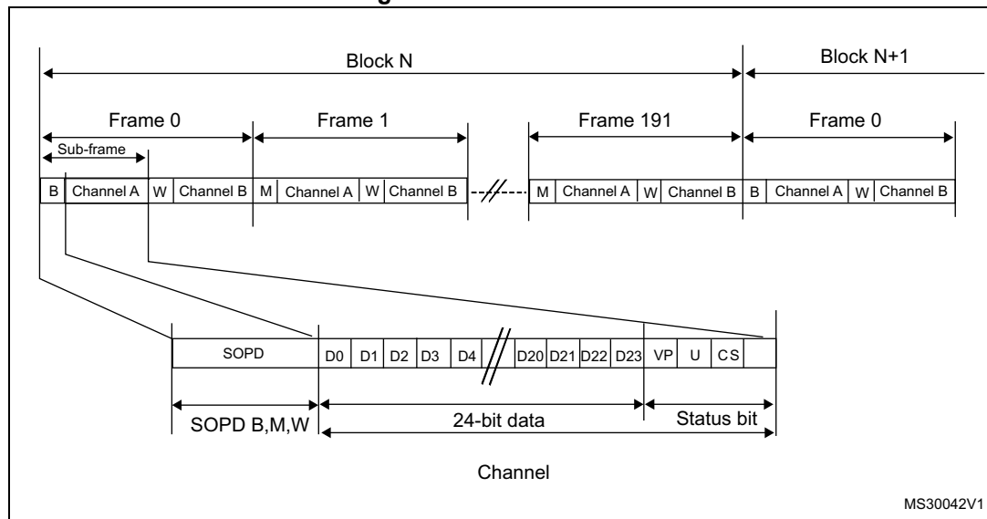
Figure 387. SPDIF format
