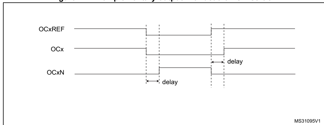
Figure 172. Complementary output with dead-time insertion
