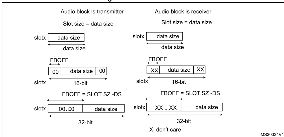
Figure 383. First bit offset
