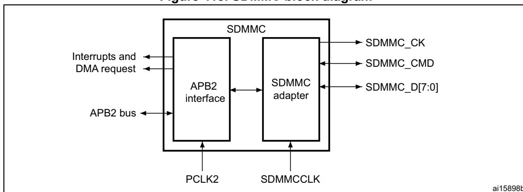
Figure 415. SDMMC block diagram
