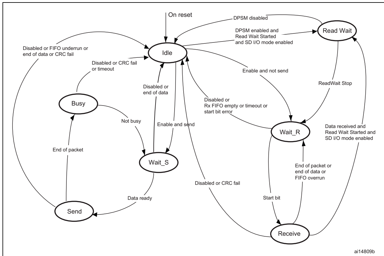
Figure 423. Data path state machine (DPSM)
