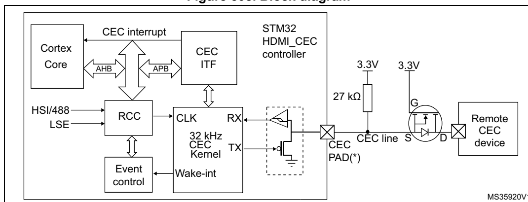
Figure 508. Block diagram
