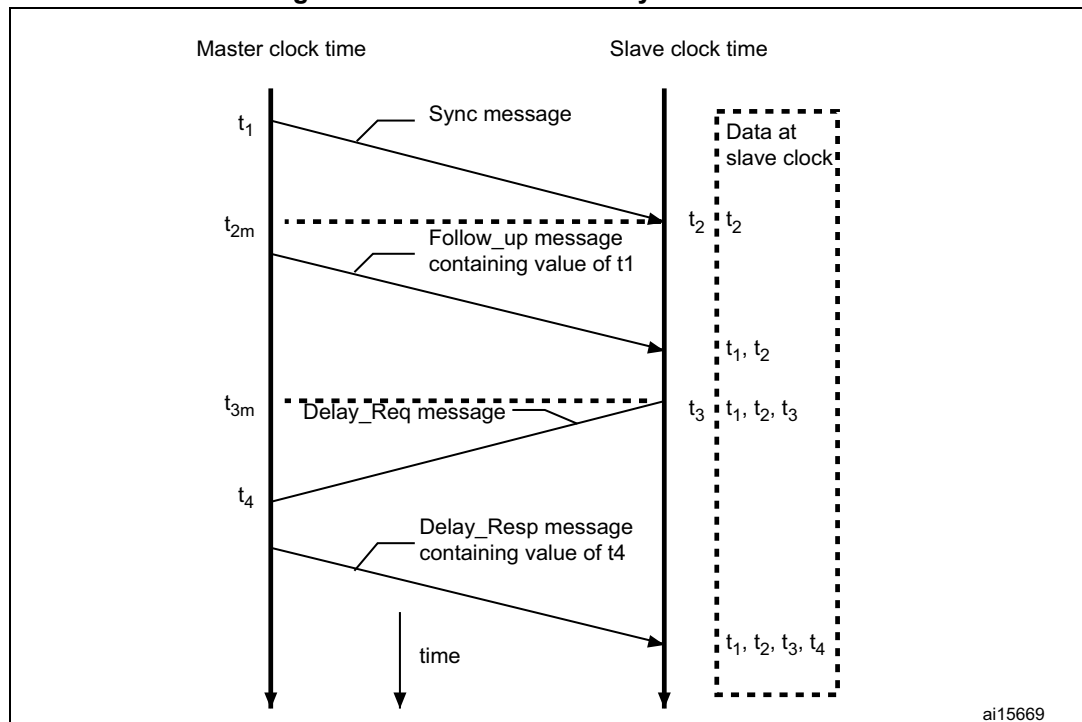
Figure 494. Networked time synchronization
