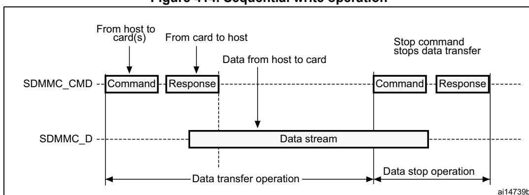
Figure 414. Sequential write operation
