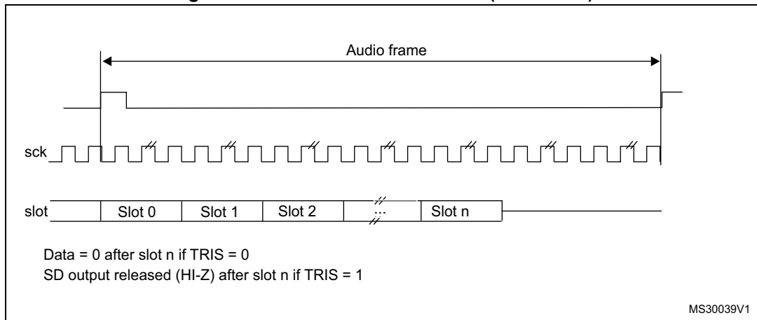
Figure 381. FS role is start of frame (FSDEF = 0)
