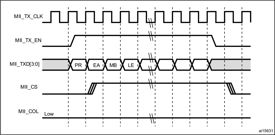
Figure 485. Transmission with no collision
