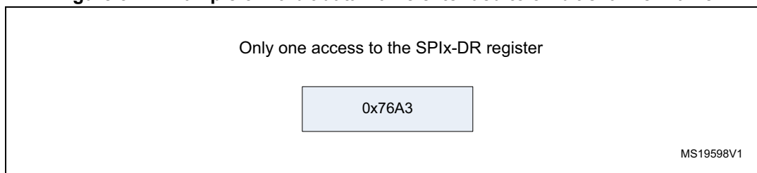
Figure 372. Example of 16-bit data frame extended to 32-bit channel frame
