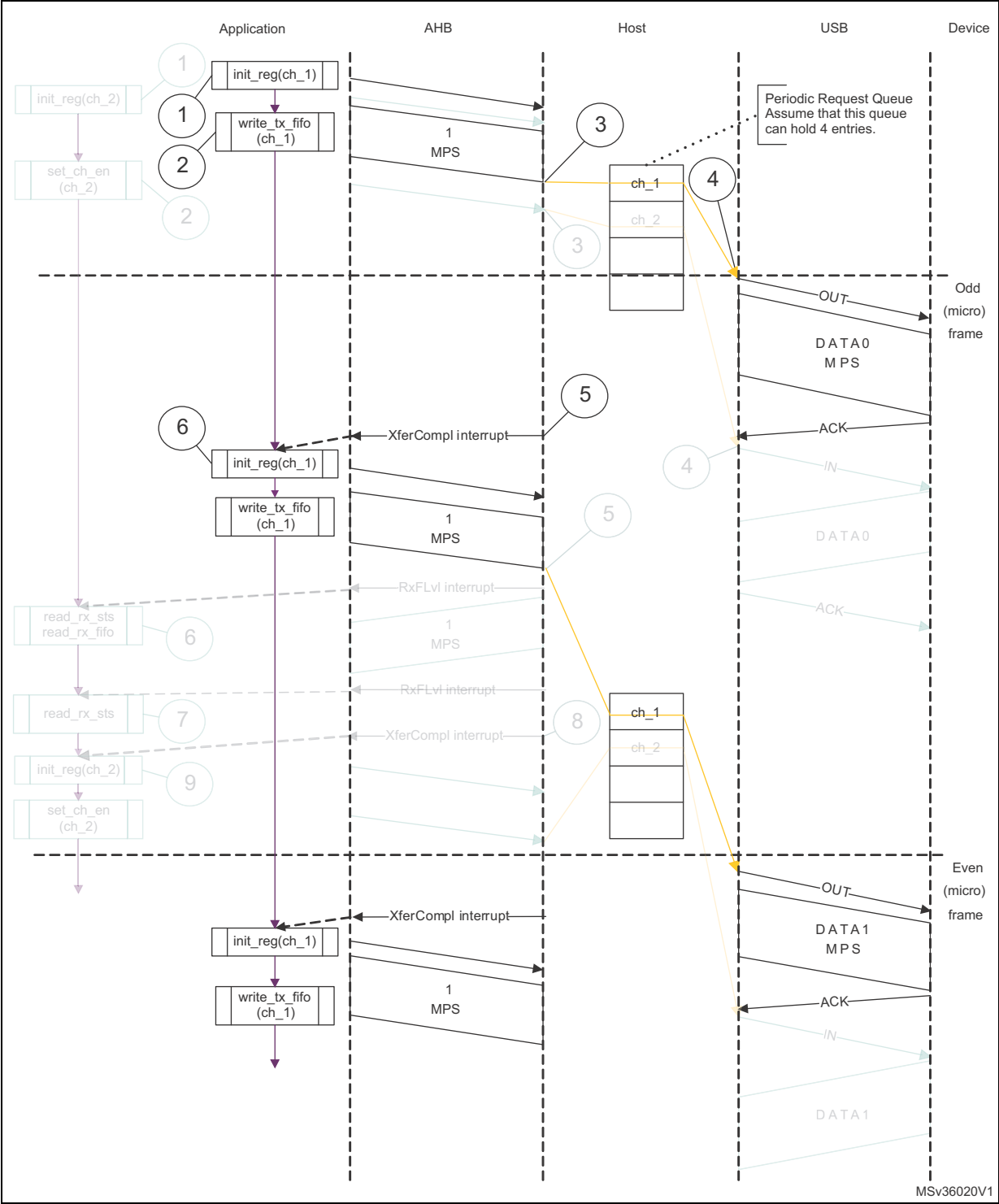
Figure 454. Normal interrupt OUT
