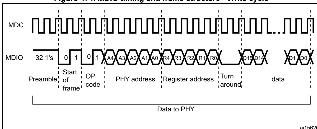
Figure 474. MDIO timing and frame structure - Write cycle
