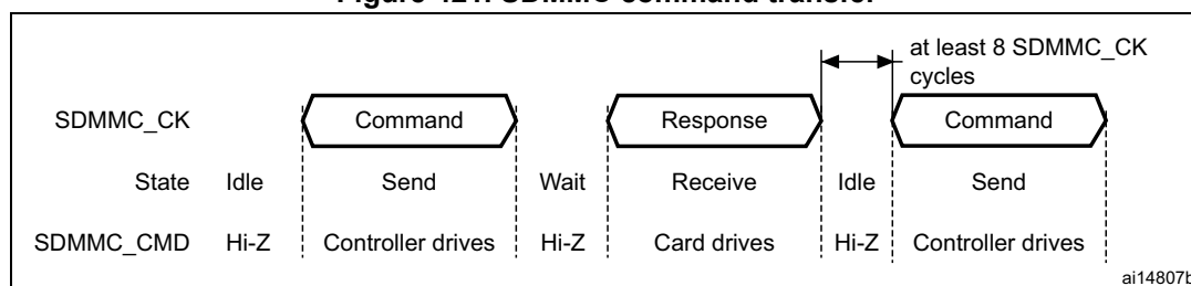
Figure 421. SDMMC command transfer
