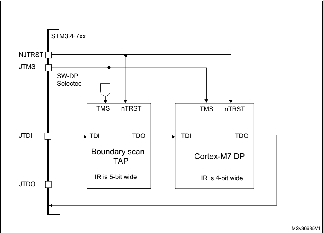
Figure 520. JTAG Debug Port connections
