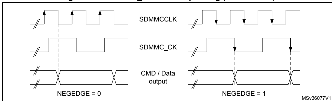
Figure 418. SDMMC_CLK clock dephasing (BYPASS = 0)
