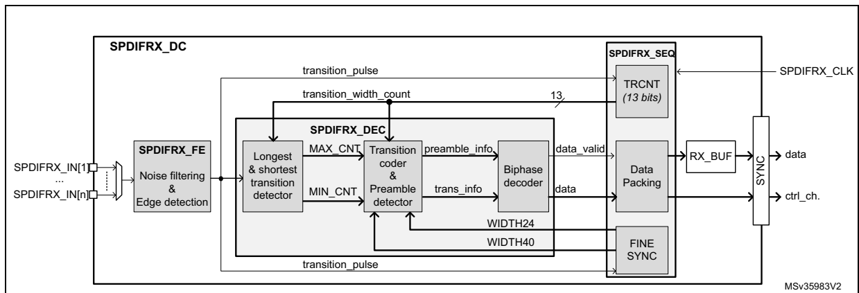
Figure 399.SPDIFRX_DC Decoder
