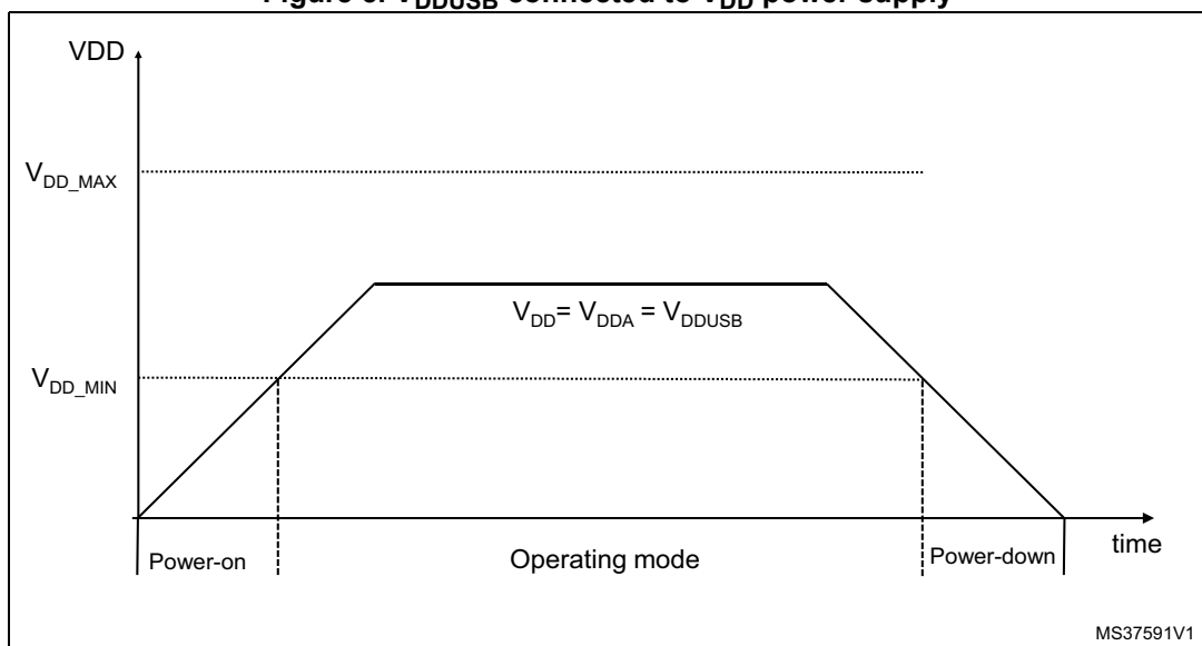
Figure 5. V_{DDUSB} connected to V_{DD} power supply
