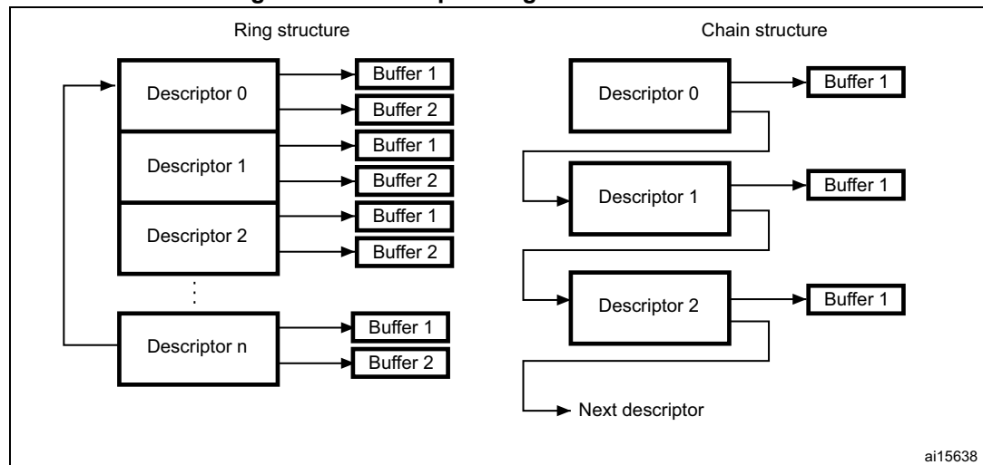
Figure 498. Descriptor ring and chain structure
