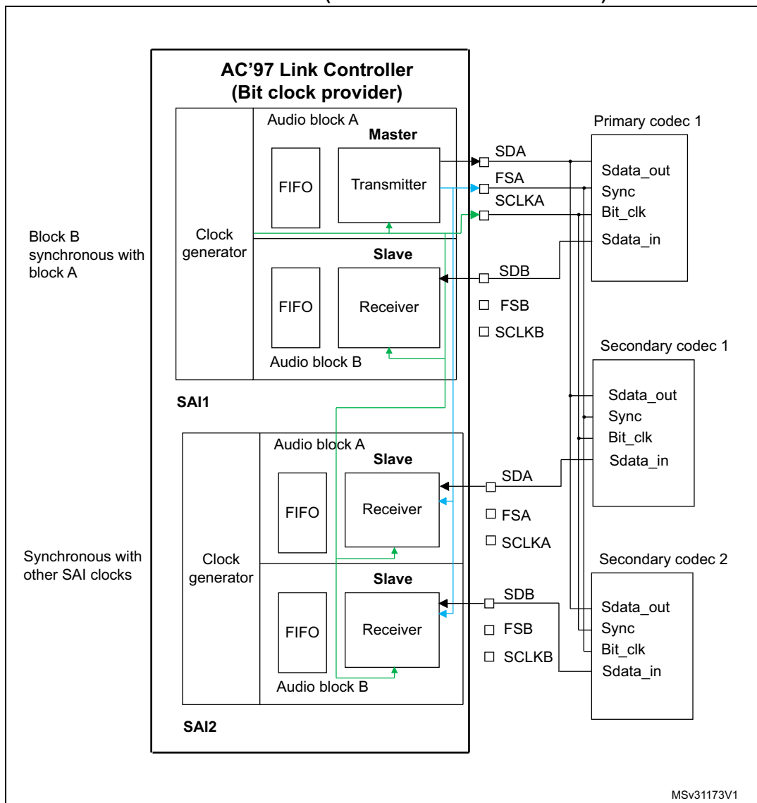
Figure 386. Example of typical AC'97 configuration on devices featuring at least 2 embedded SAIs (three external AC'97 decoders)
