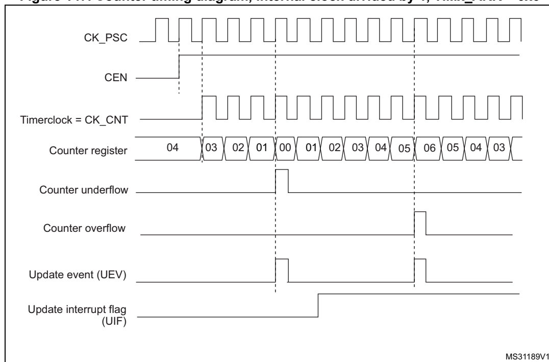
Figure 147. Counter timing diagram, internal clock divided by 1, TIMx_ARR = 0x6
