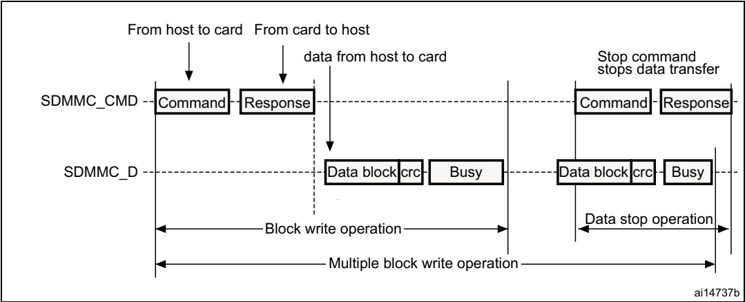
Figure 412. (Multiple) block write operation
