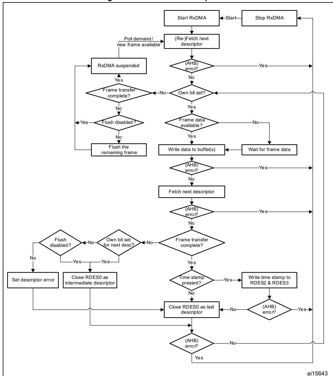
Figure 503. Receive DMA operation
