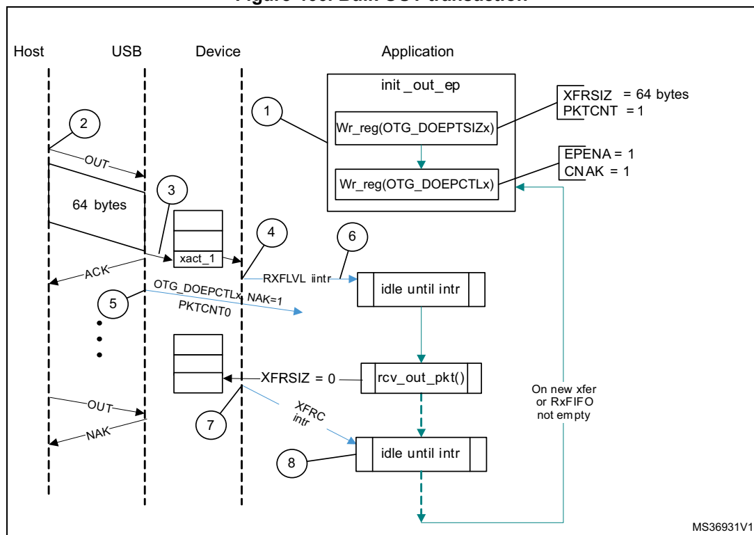
Figure 466. Bulk OUT transaction
