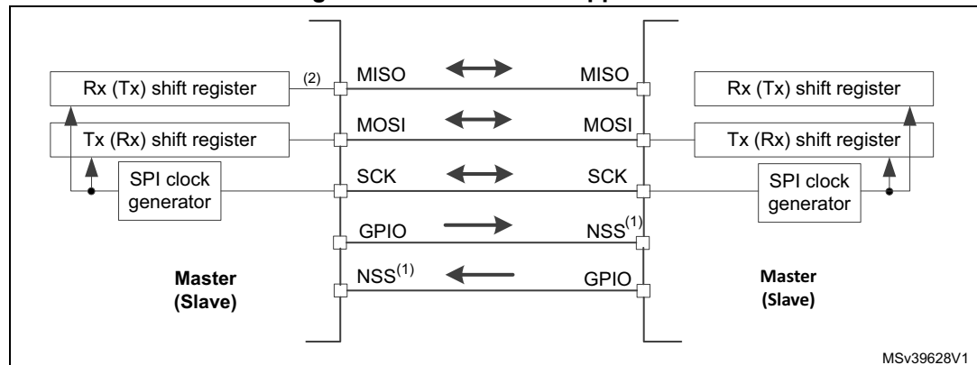
Figure 346. Multi-master application
