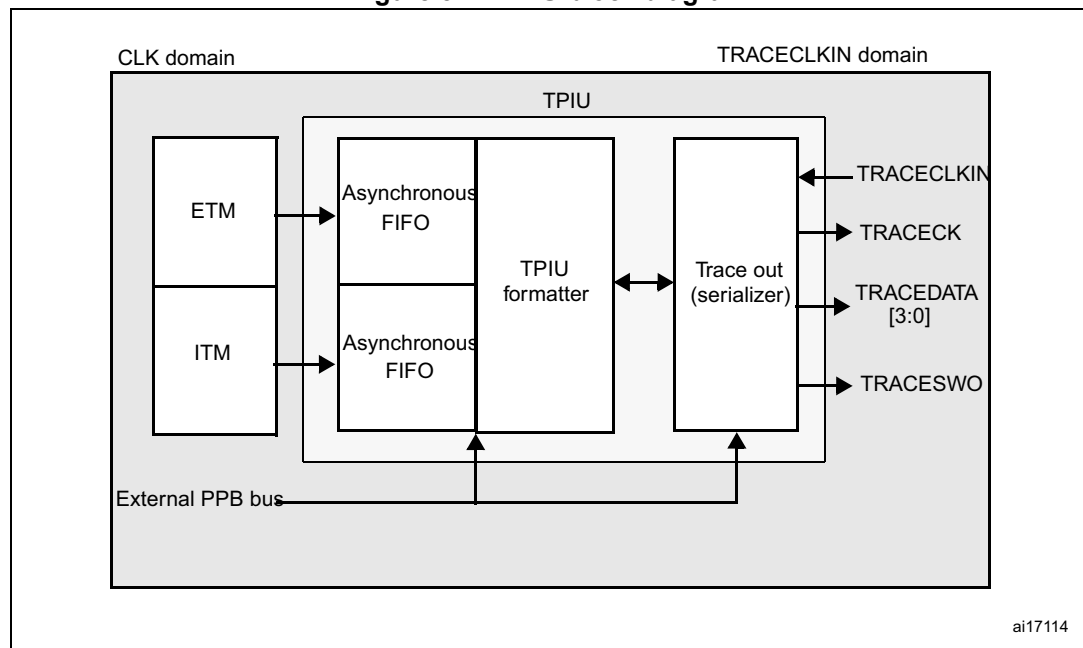
Figure 521. TPIU block diagram
