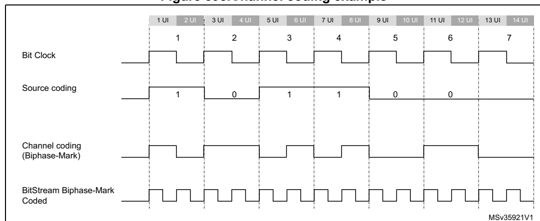
Figure 398. Channel coding example
