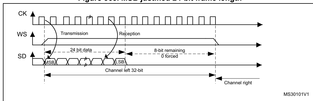
Figure 365. MSB justified 24-bit frame length
