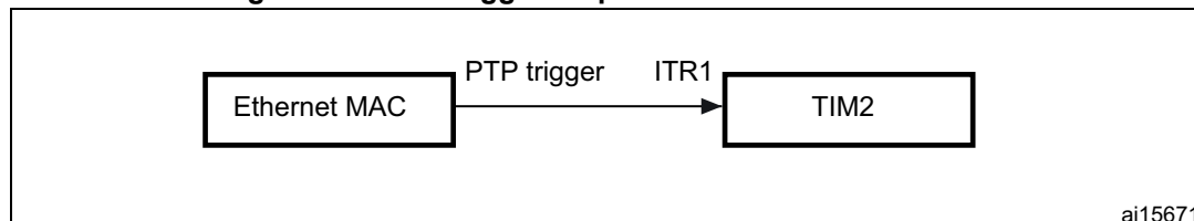
Figure 496. PTP trigger output to TIM2 ITR1 connection
