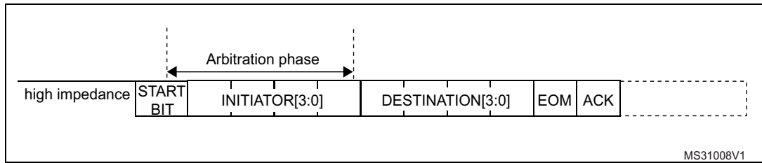
Figure 513. Arbitration phase
