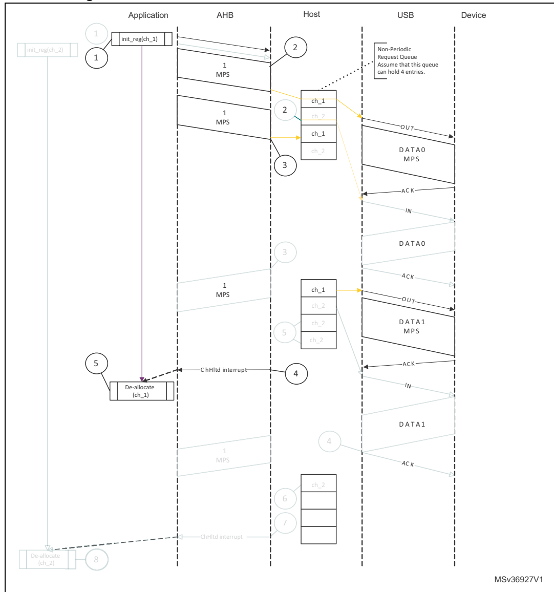
Figure 458. Normal bulk/control OUT/SETUP transactions - DMA
