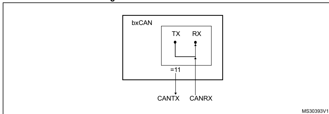
Figure 427. bxCAN in silent mode
