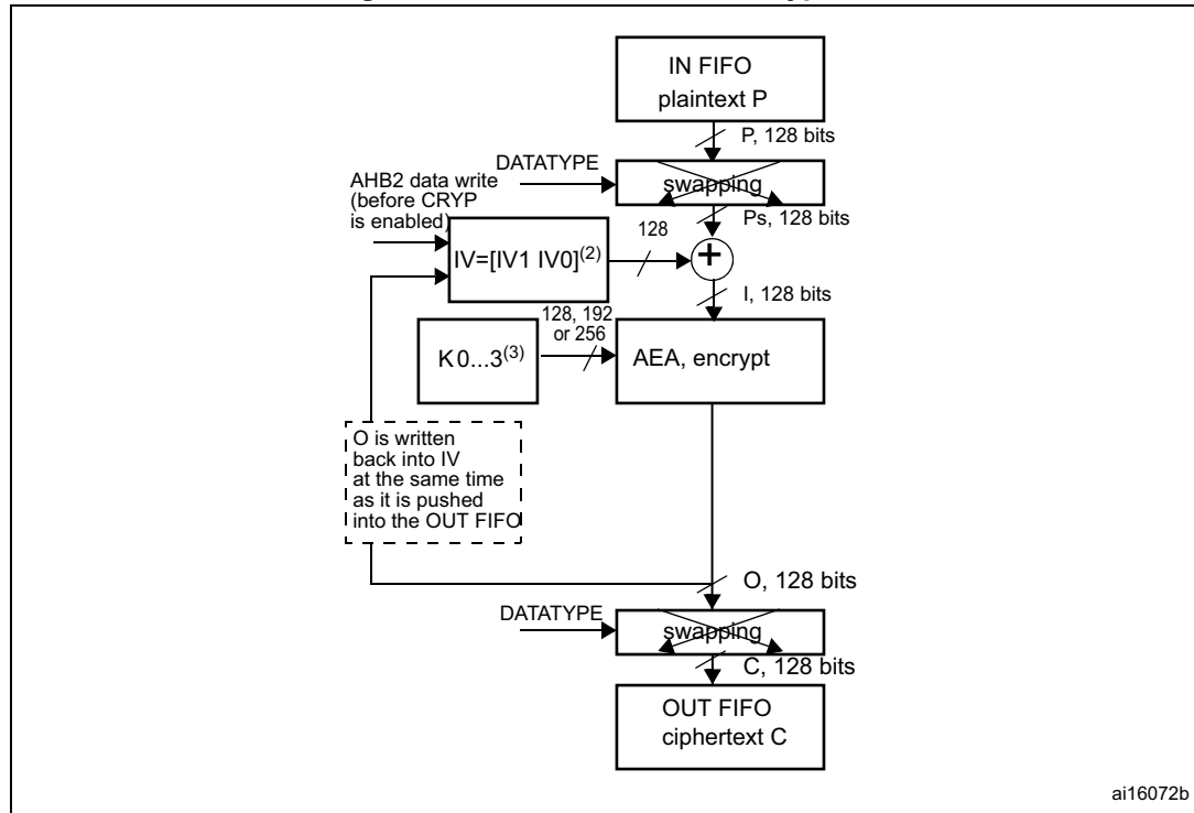
Figure 123. AES-CBC mode encryption
