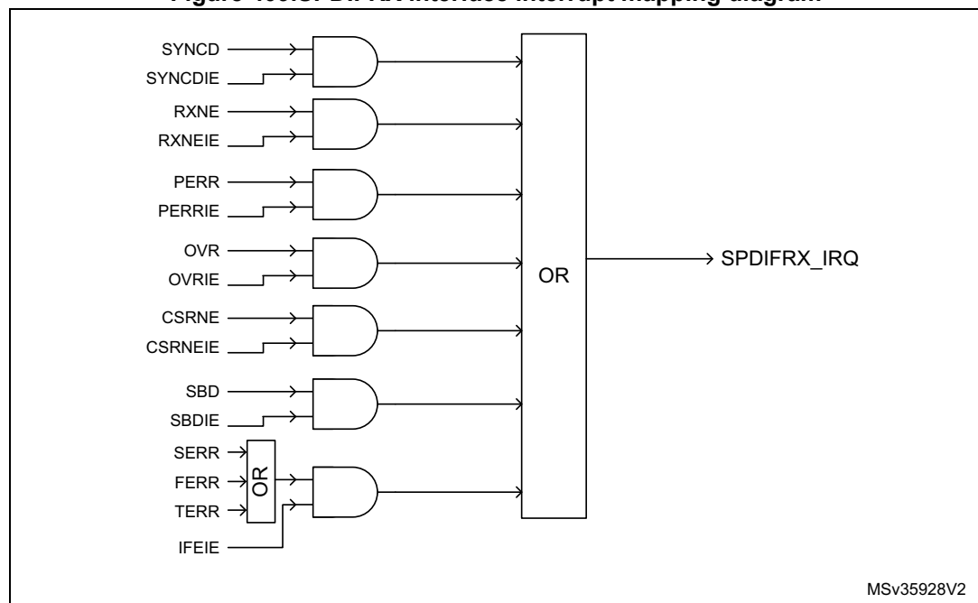
Figure 409. SPDIFRX interface interrupt mapping diagram
