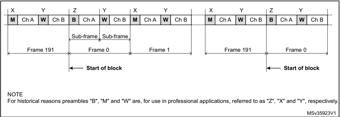
Figure 396.S/PDIF block format
