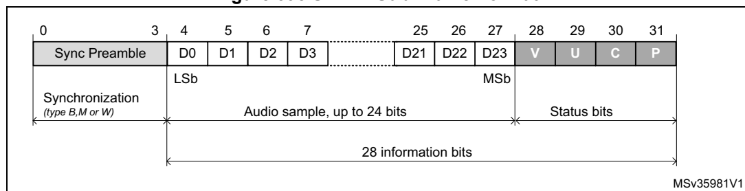
Figure 395.S/PDIF Sub-Frame Format
