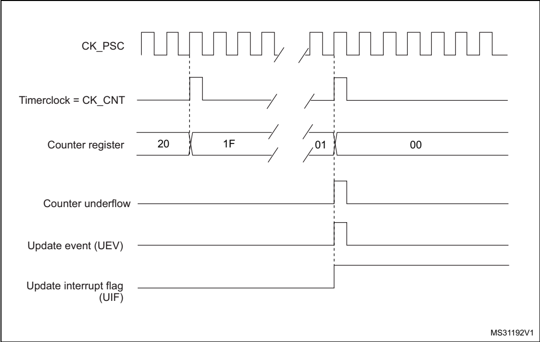
Figure 208. Counter timing diagram, internal clock divided by N
