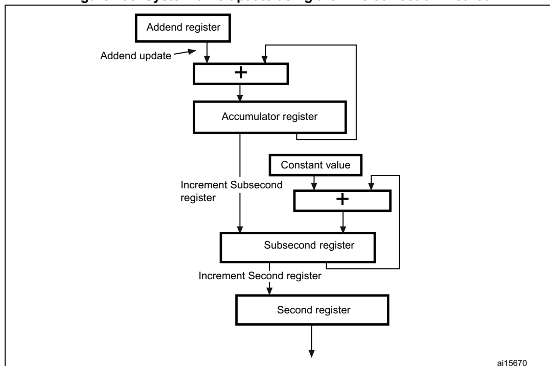
Figure 495. System time update using the Fine correction method
