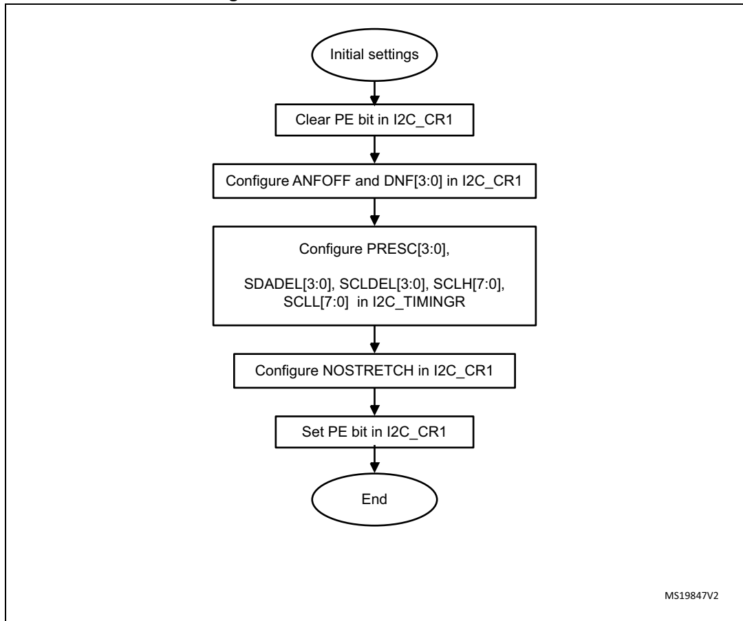
Figure 288. I2C initialization flowchart
