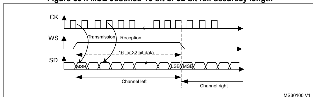
Figure 364. MSB Justified 16-bit or 32-bit full-accuracy length
