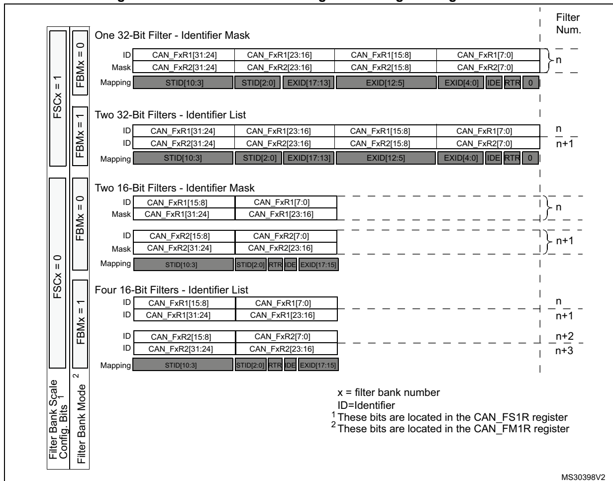
Figure 432. Filter bank scale configuration - register organization
