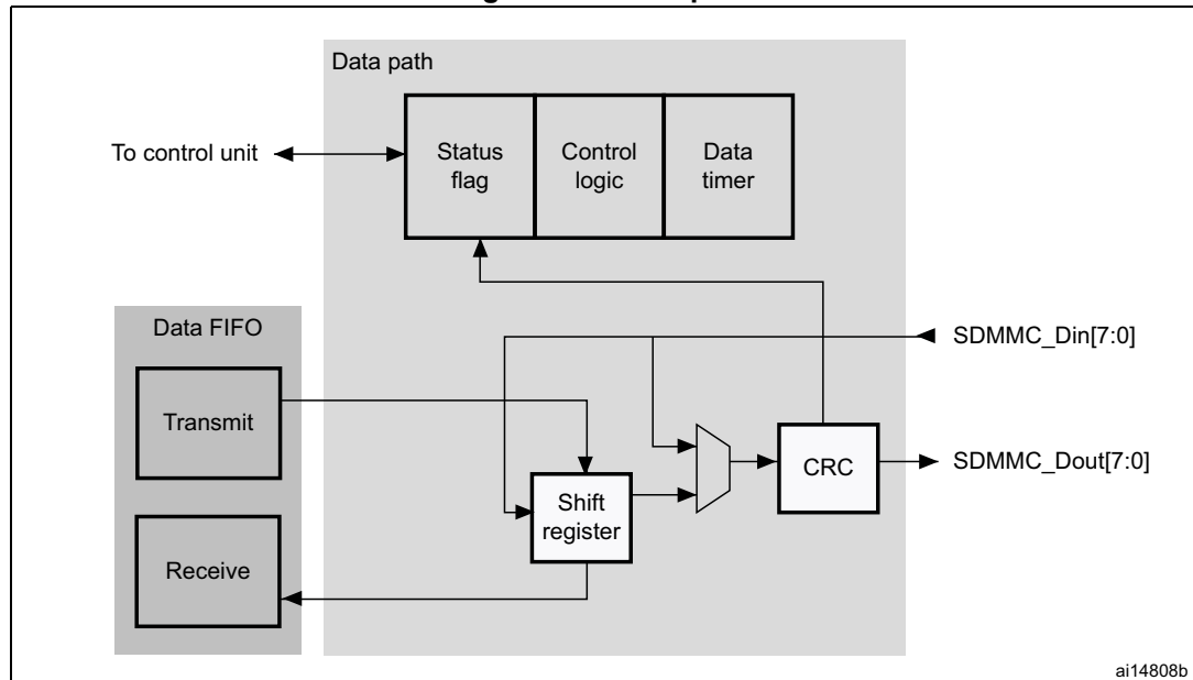
Figure 422. Data path
