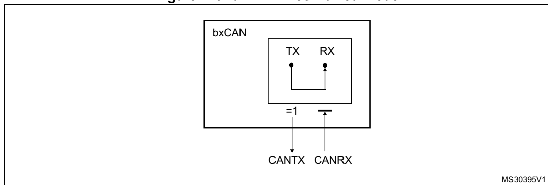
Figure 429. bxCAN in combined mode
