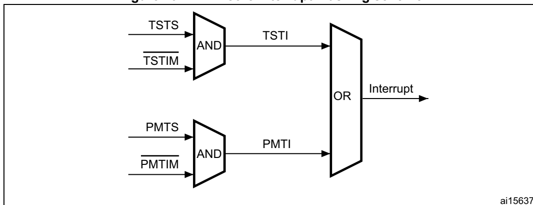
Figure 492. MAC core interrupt masking scheme
