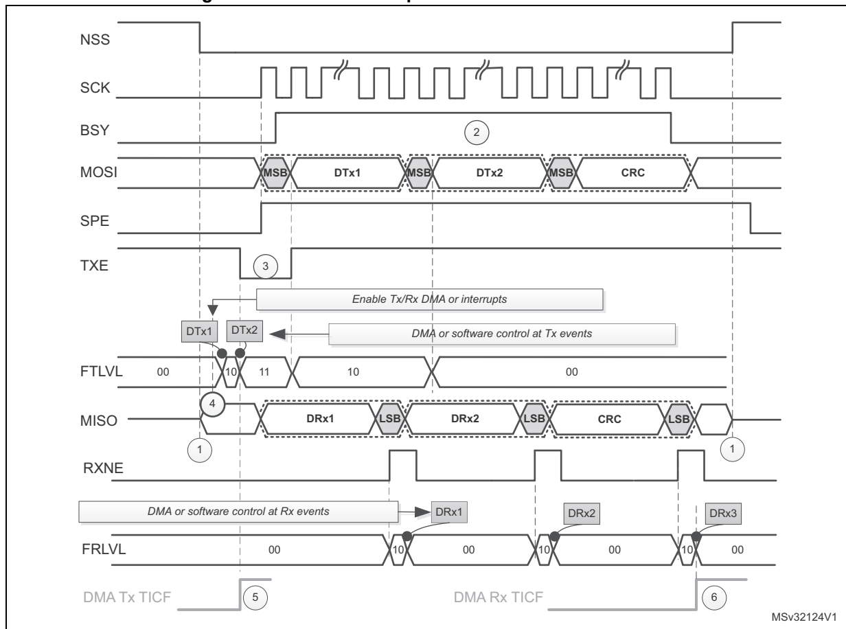
Figure 353. Master full duplex communication with CRC
