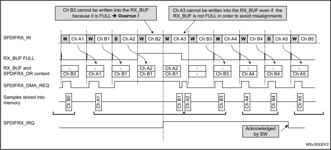
Figure 408.S/PDIF overrun error when RXSTEO = 1
