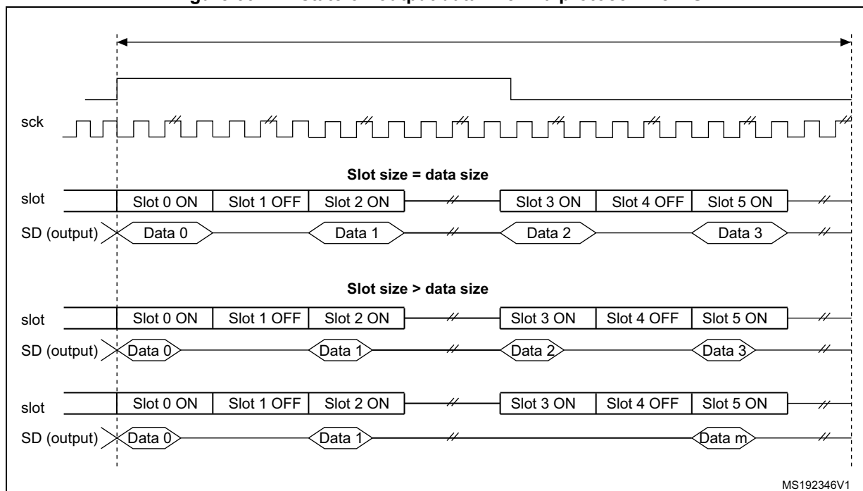
Figure 391. Tristate on output data line in a protocol like I2S
