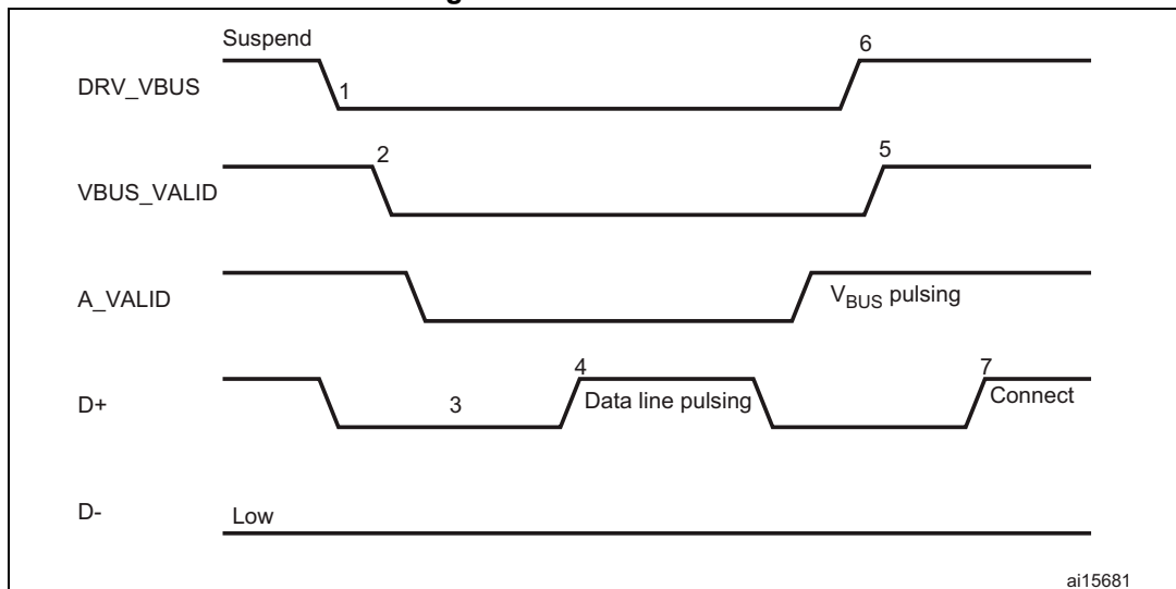
Figure 468. A-device SRP
