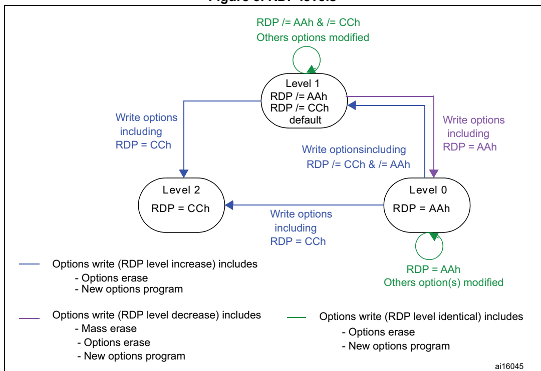
Figure 3. RDP levels
