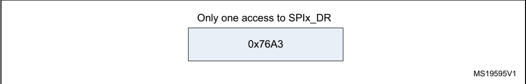
Figure 363. Example of 16-bit data frame extended to 32-bit channel frame
