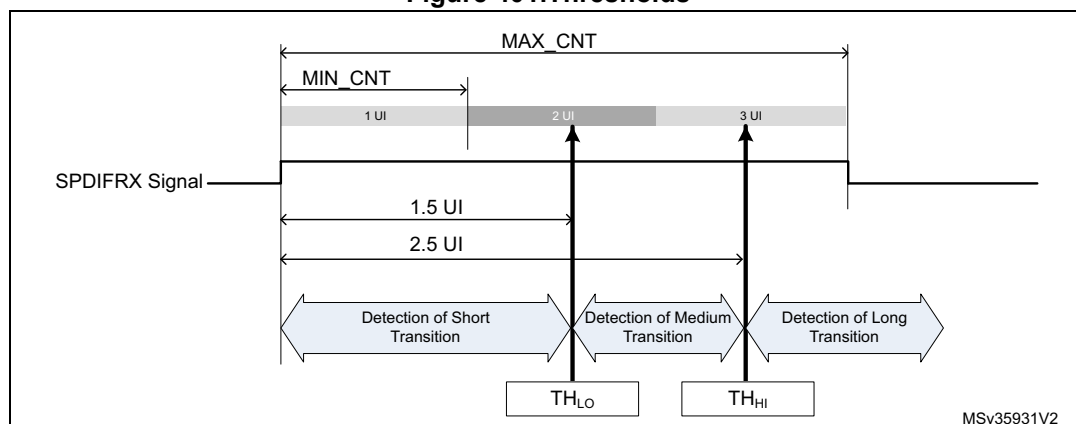
Figure 401. Thresholds
