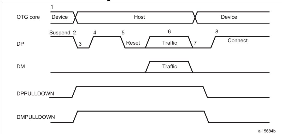
Figure 471. B-device HNP
