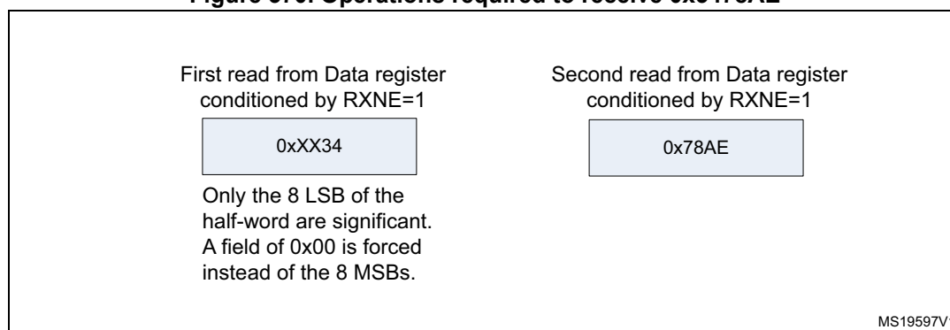
Figure 370. Operations required to receive 0x3478AE
