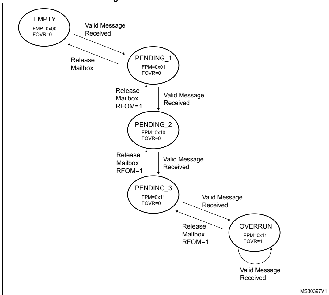
Figure 431. Receive FIFO states
