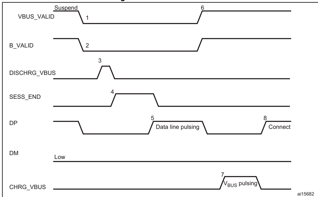
Figure 469. B-device SRP
