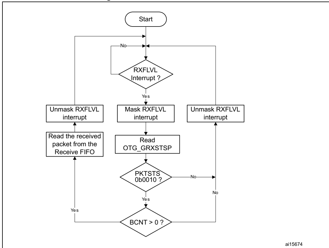
Figure 451. Receive FIFO read task
