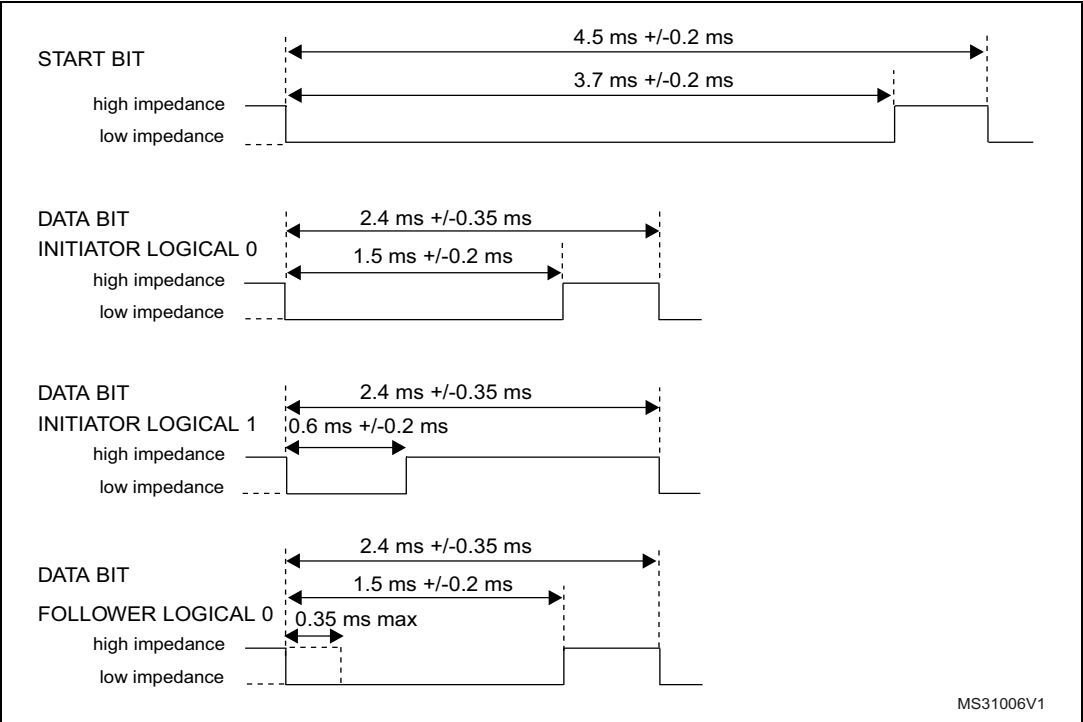
Figure 511. Bit timings
