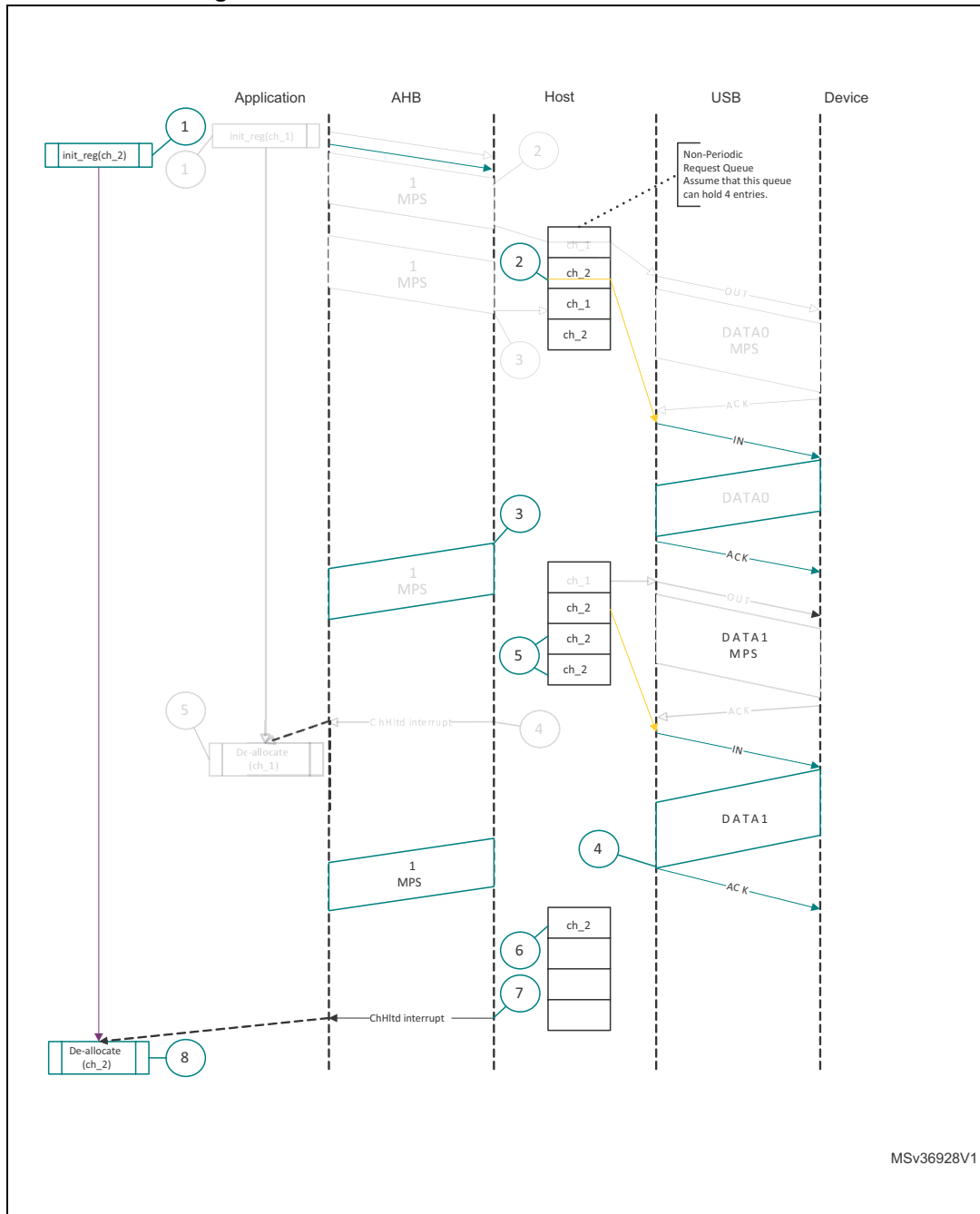
Figure 459. Normal bulk/control IN transaction - DMA
