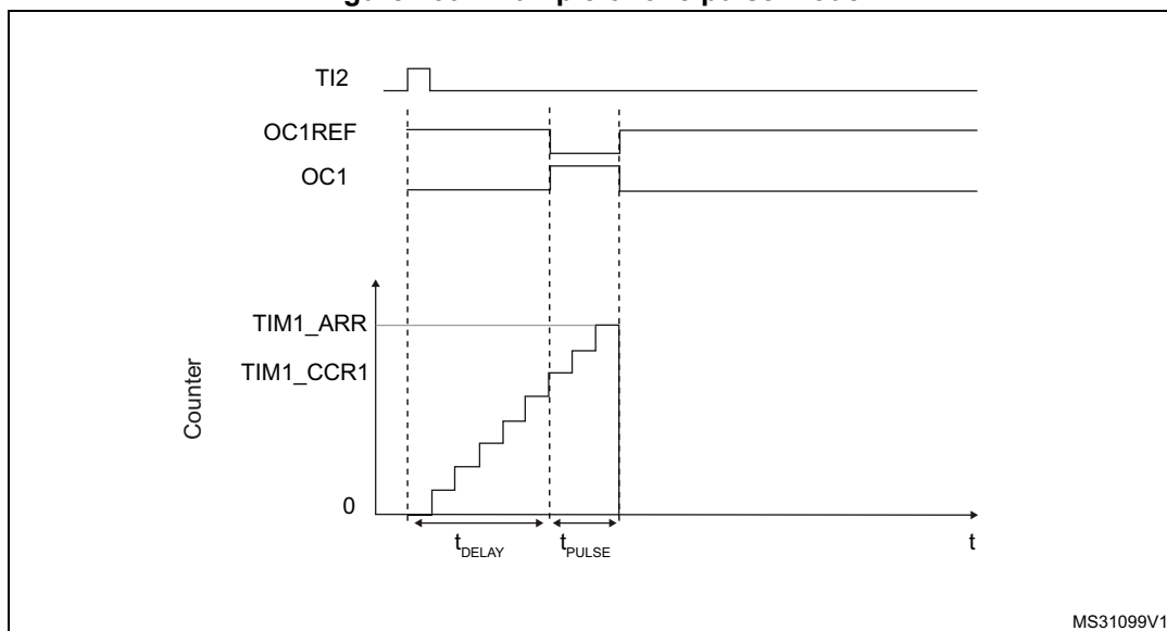
Figure 260. Example of one pulse mode.
