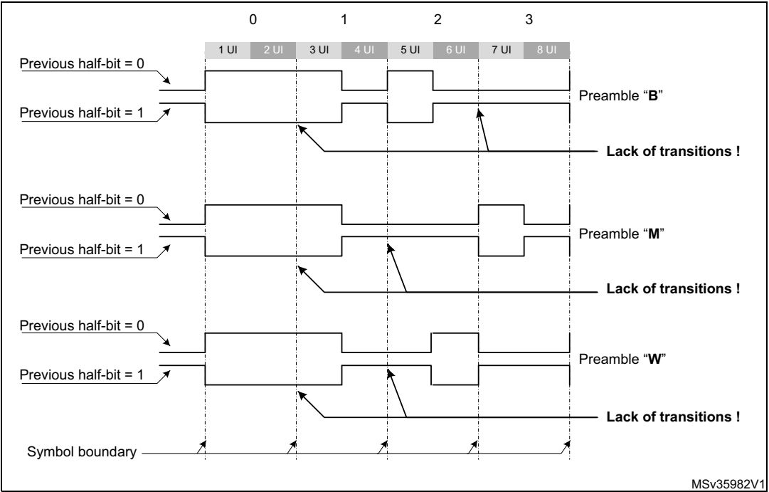
Figure 397.S/PDIF Preambles
