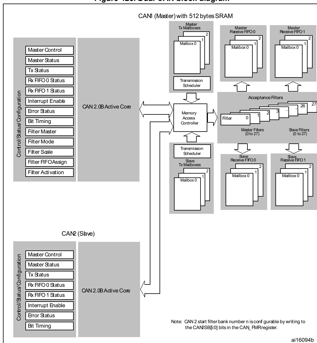
Figure 425. Dual CAN block diagram
