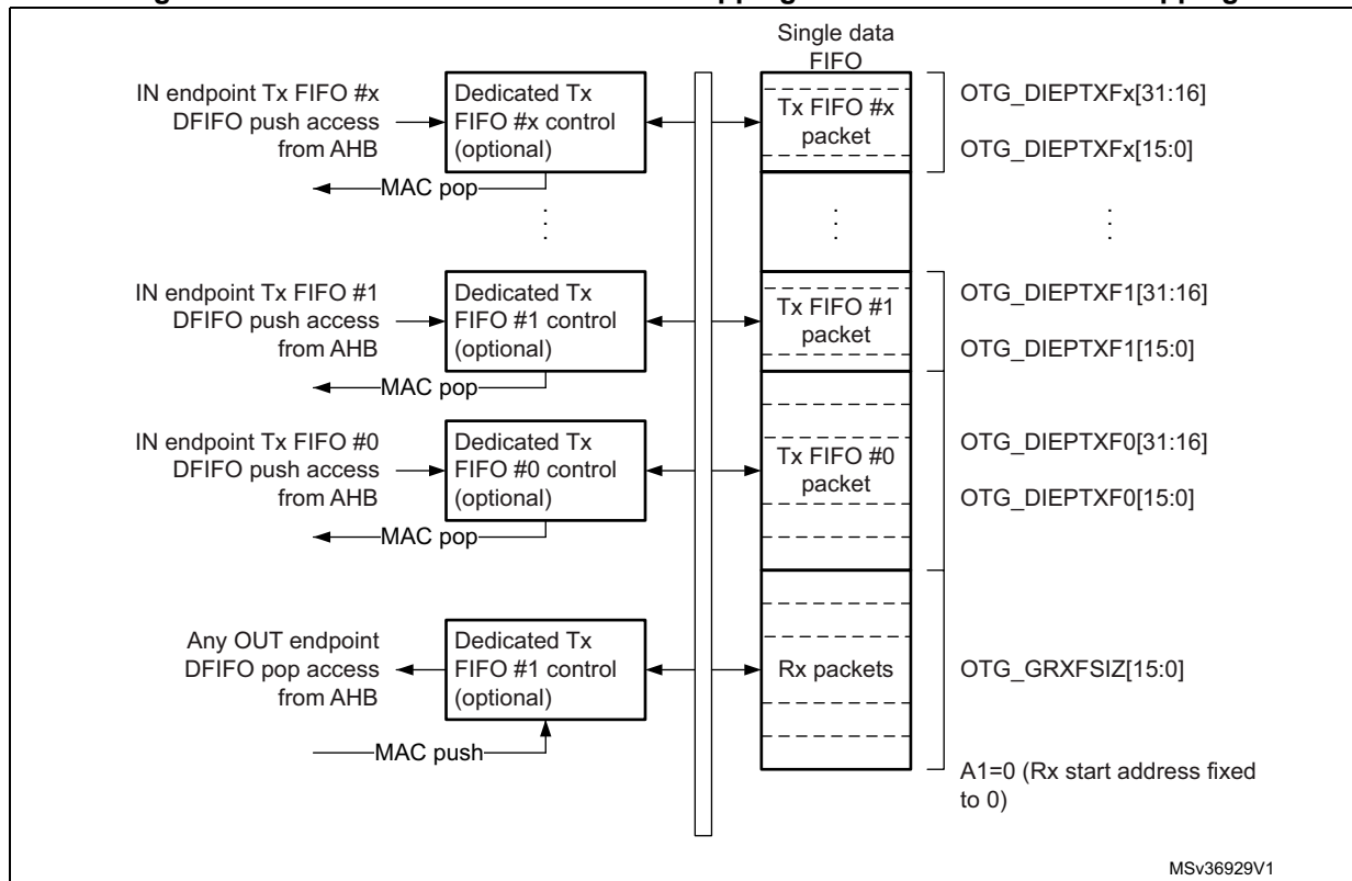
Figure 447. Device-mode FIFO address mapping and AHB FIFO access mapping
