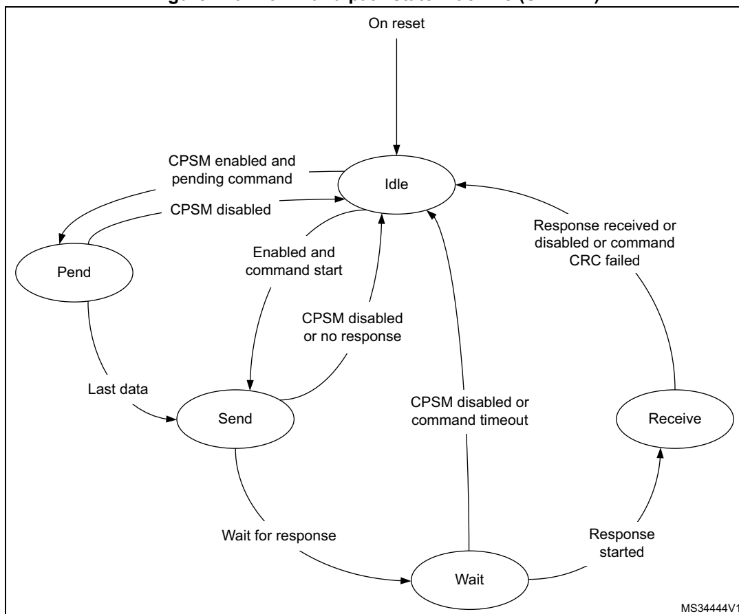
Figure 420. Command path state machine (SDMMC)
