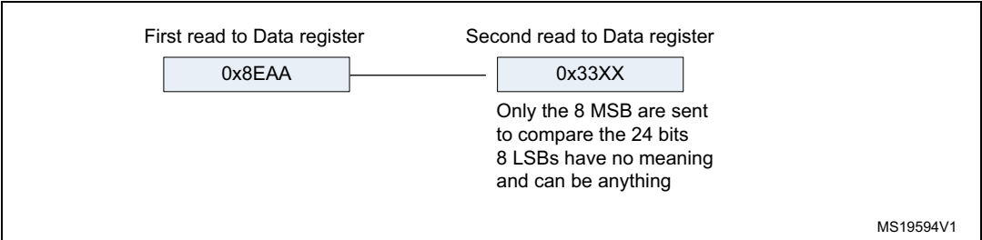
Figure 361. Receiving 0x8EAA33
