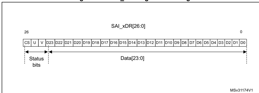
Figure 388. SAI_xDR register ordering
