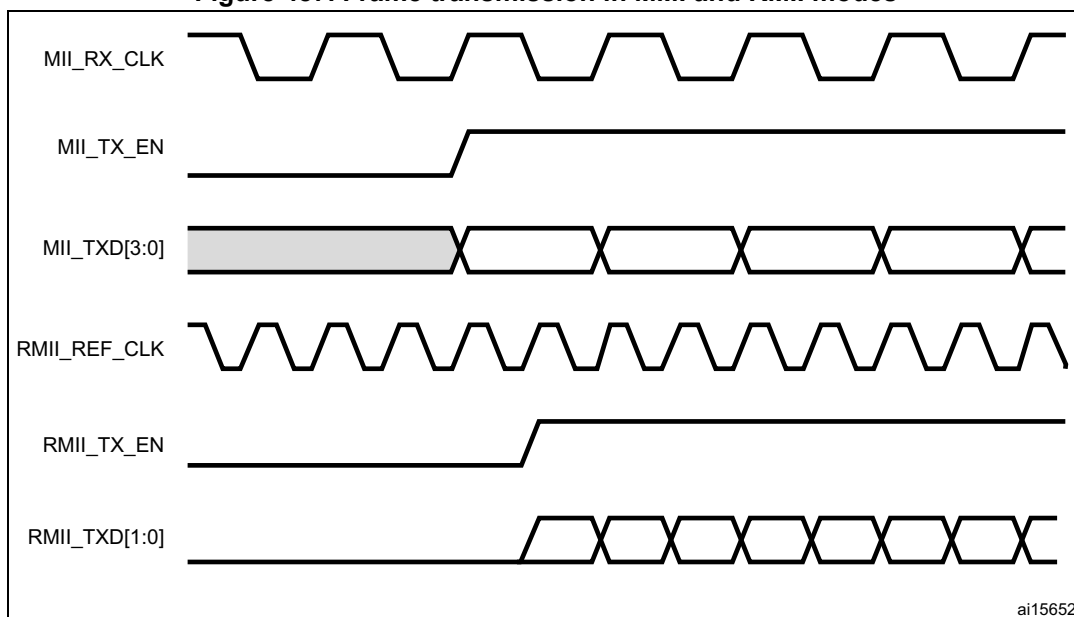
Figure 487. Frame transmission in MII and RMII modes
