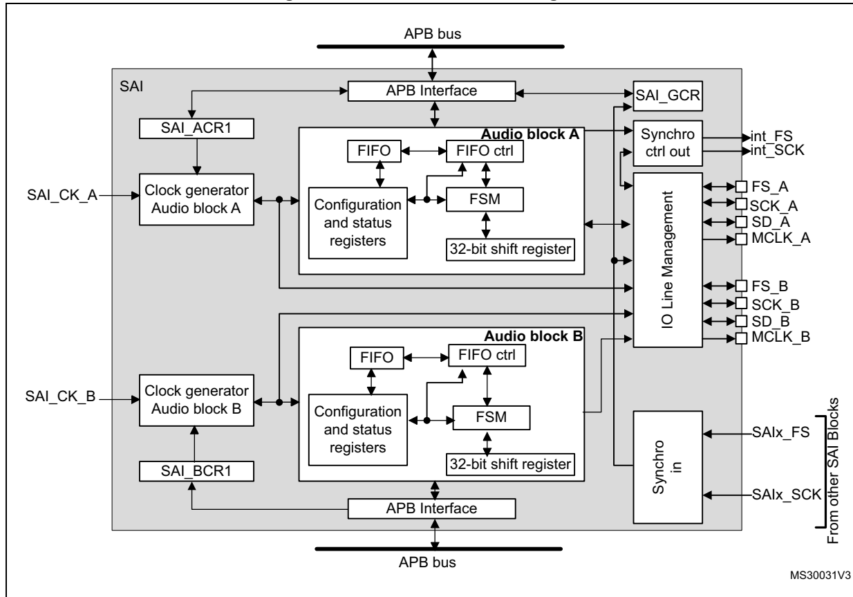
Figure 378. Functional block diagram
