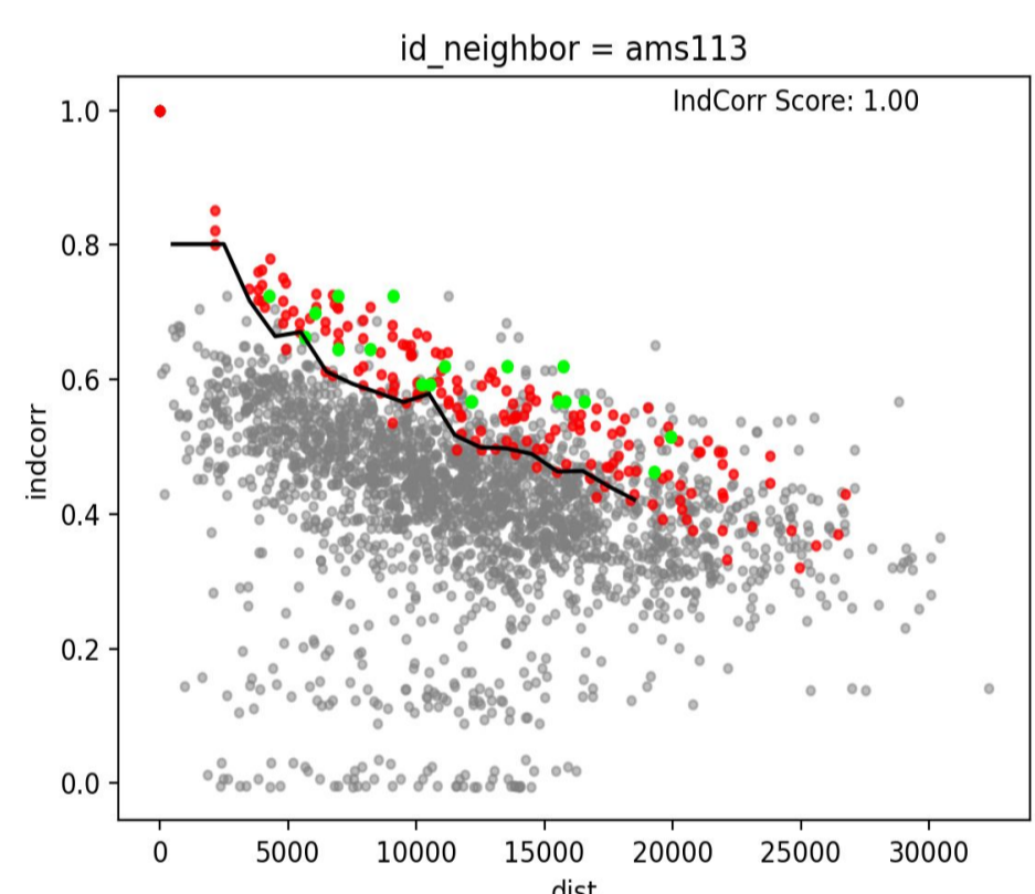
Fig 1.1: Example of a PWS with a perfect skill score as the indicator correlation in all ranges bins is at least as good as the reference
