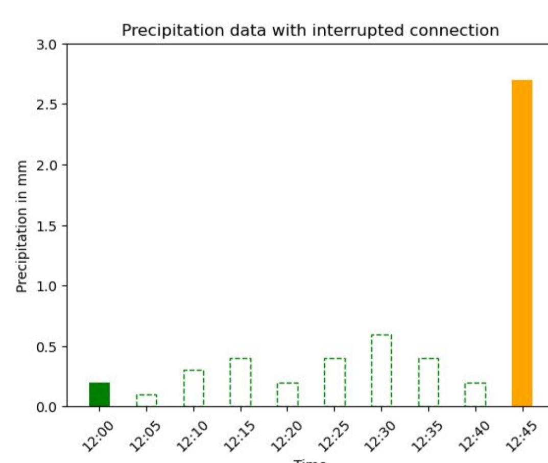
Fig 2.1: The dashed green bins show the true rainfall during an interrupted connection. These are NaN in the PWS data. The orange bin shows the data as it is transmitted after the connection is reestablished.
