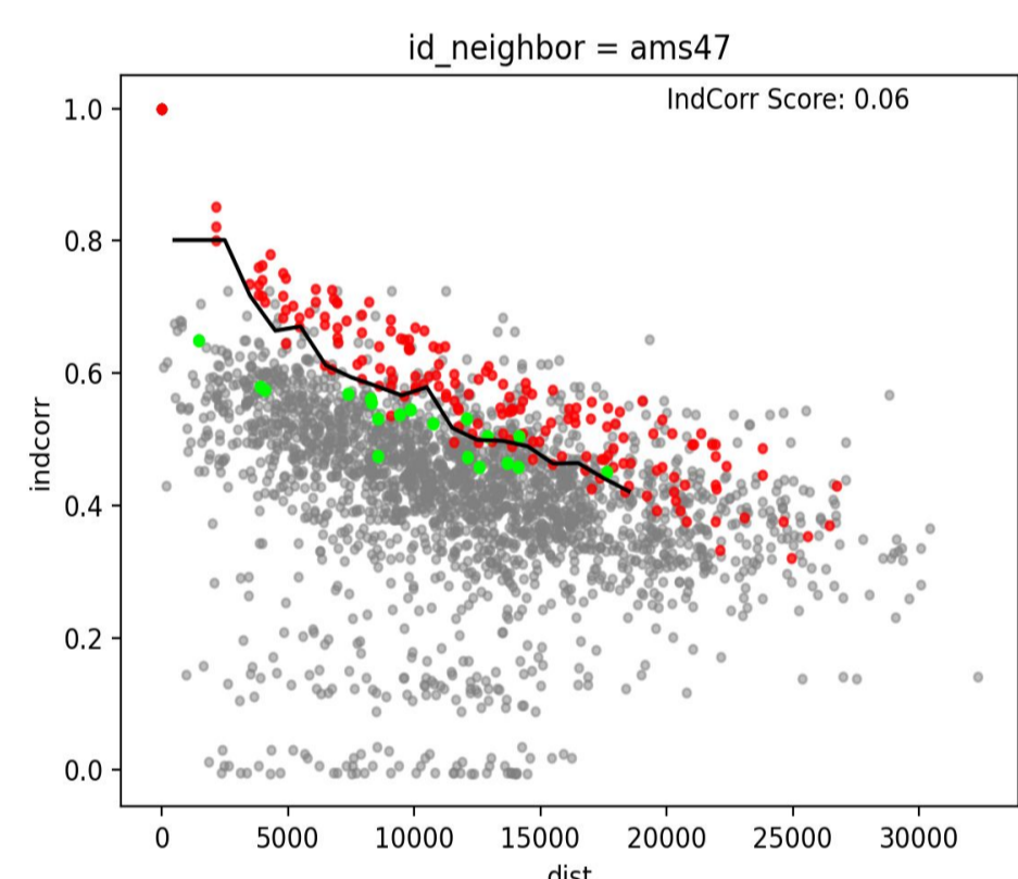
Fig 1.3: Example of a PWS with low skill score. Here, the indicator correlation is below the reference except for the distant range bins which have a low weight resulting in a low skill score
