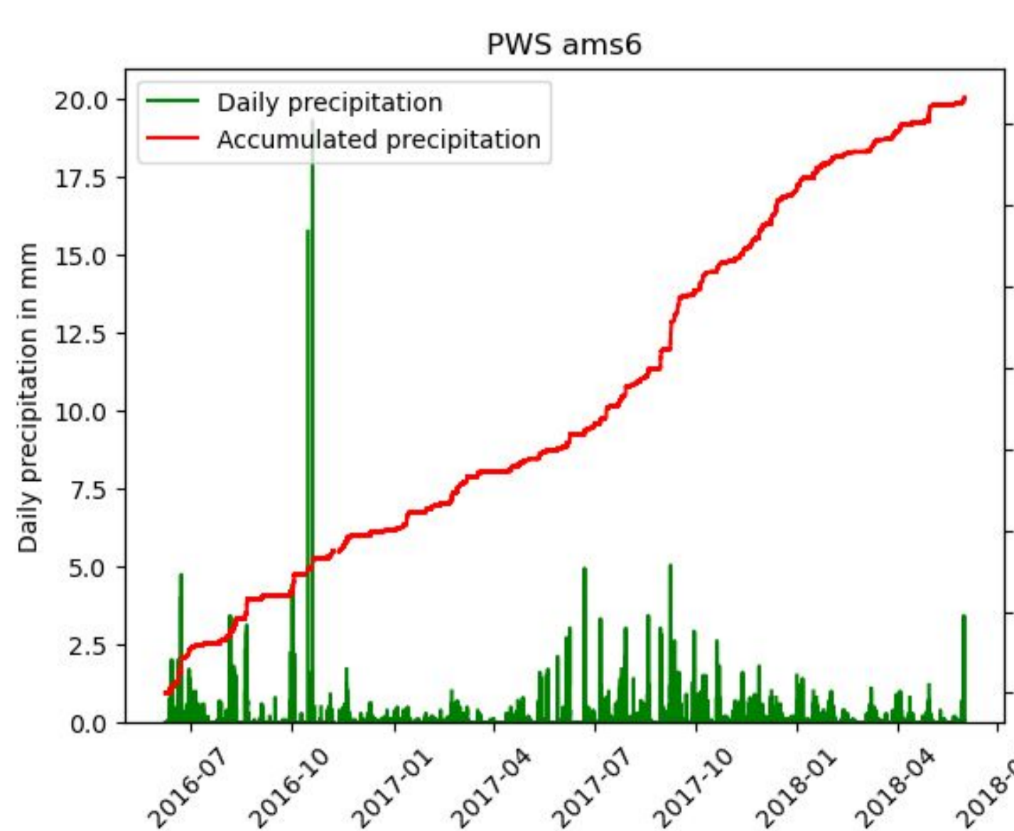
Fig 2.2: PWS rainfall time series before (left) and after (right) the application of the peak removal filter.
