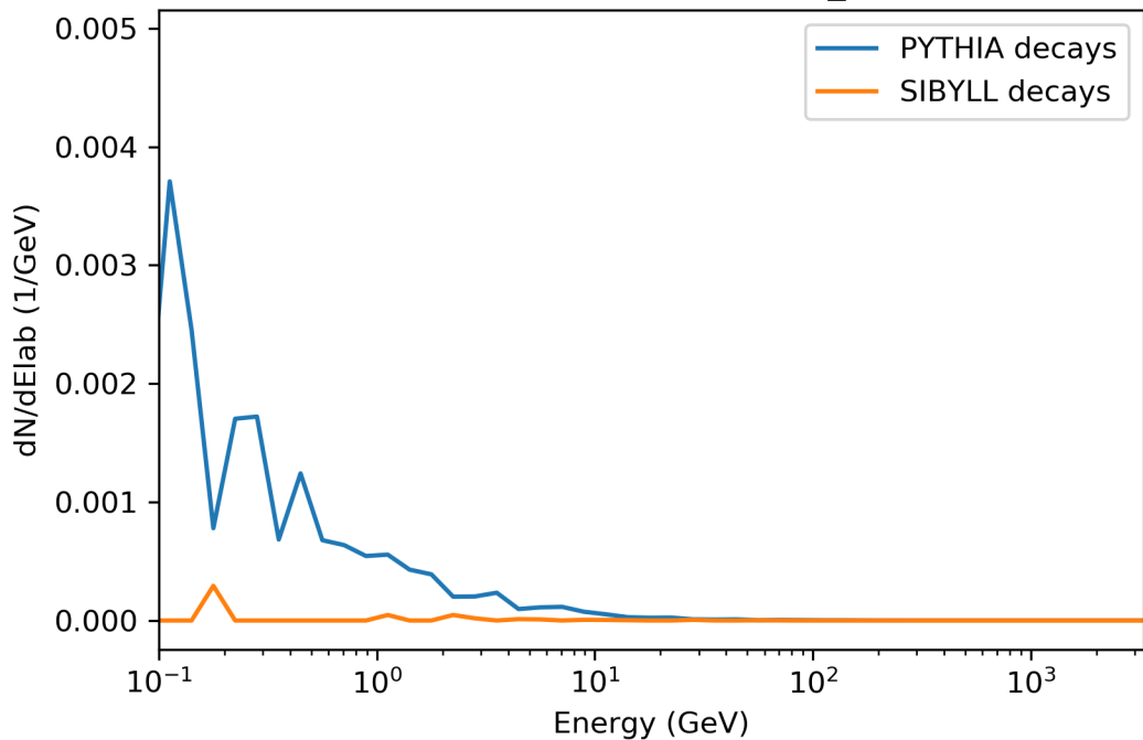
3000 GeV, SIBYLL23C, PDG_ID=12
