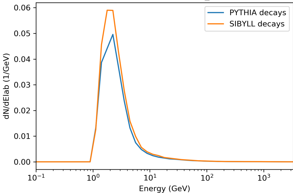
3000 GeV, SIBYLL23C, PDG_ID=3122
