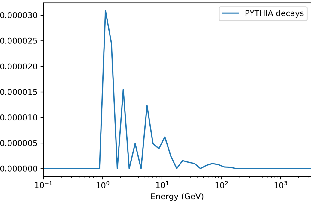
3000 GeV, SIBYLL23C, PDG_ID=16
